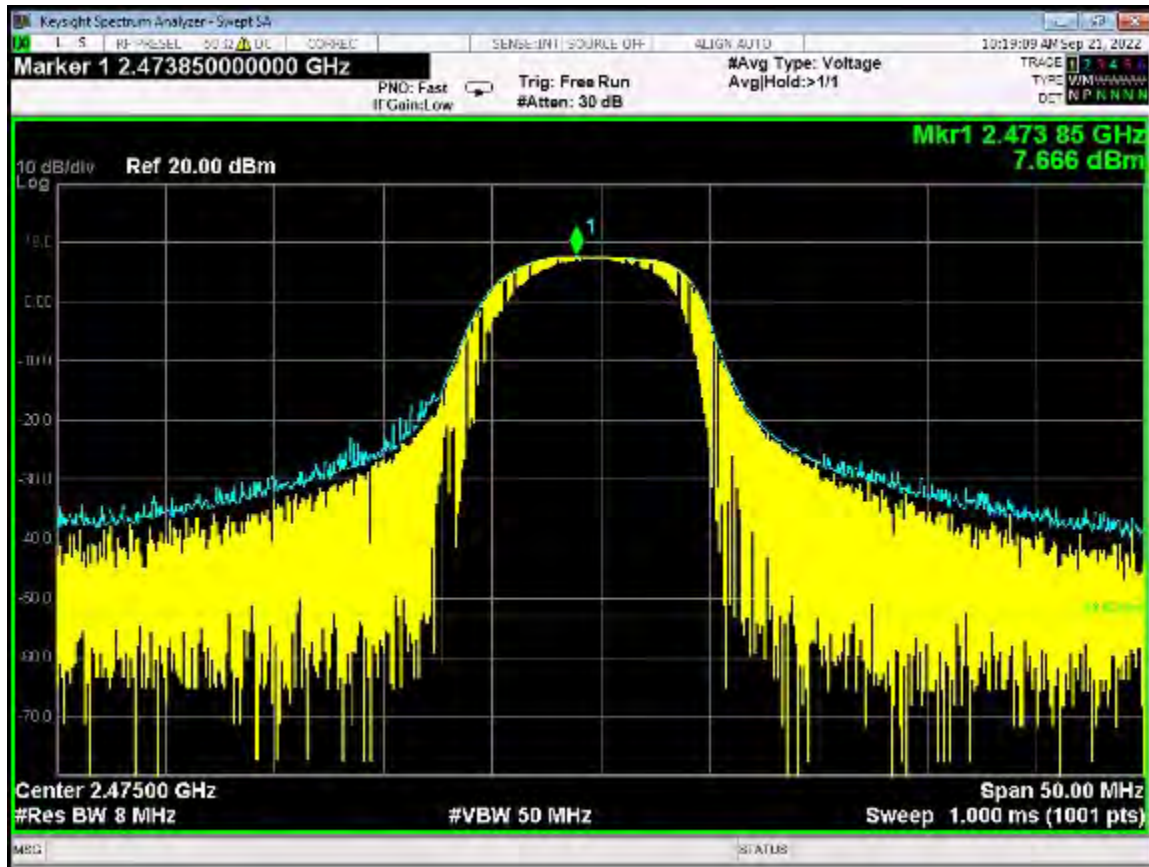
Peak Power Output – ANT 0 – 2475 MHz
