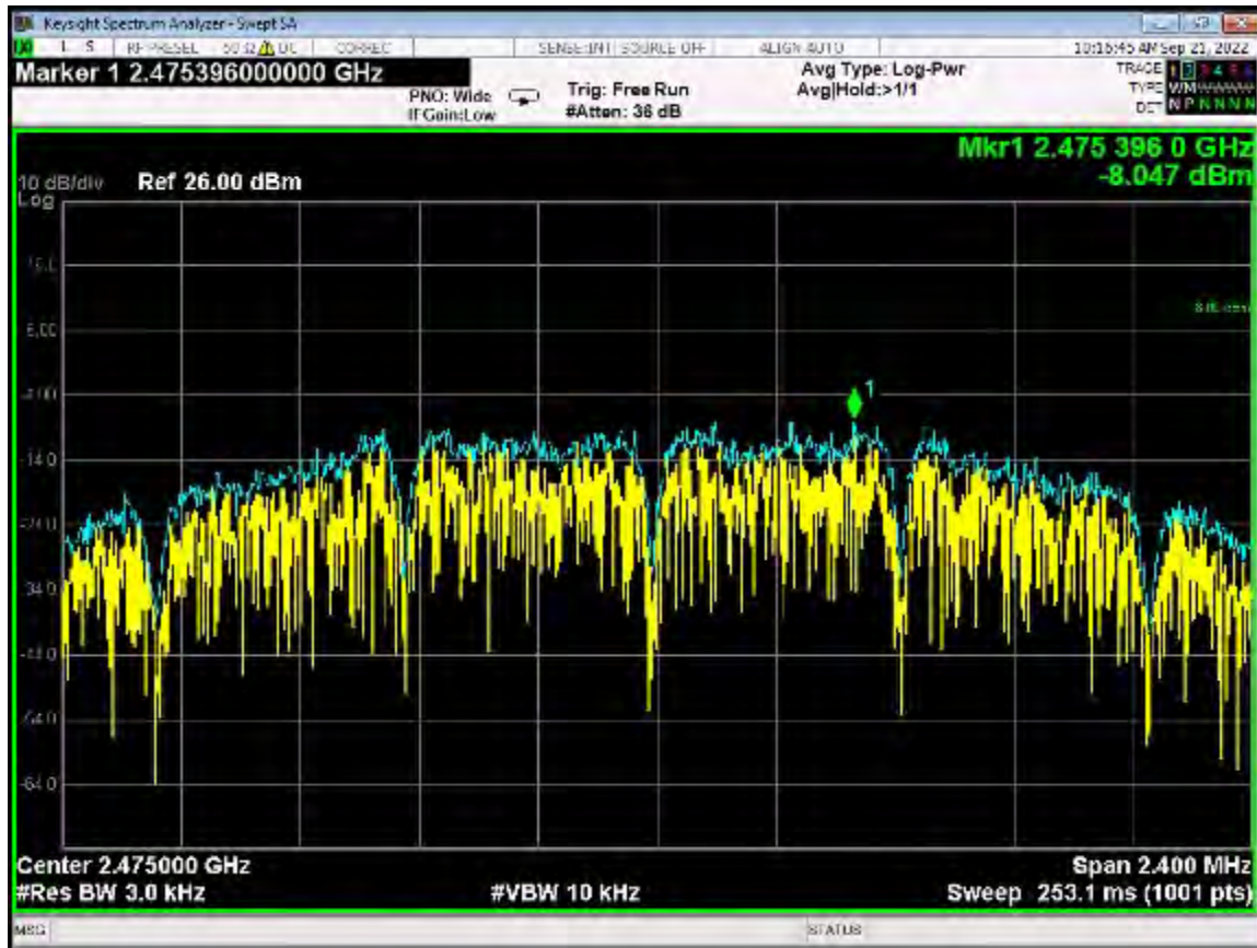
Special Density Output - ANT 0 - 2475 MHz
