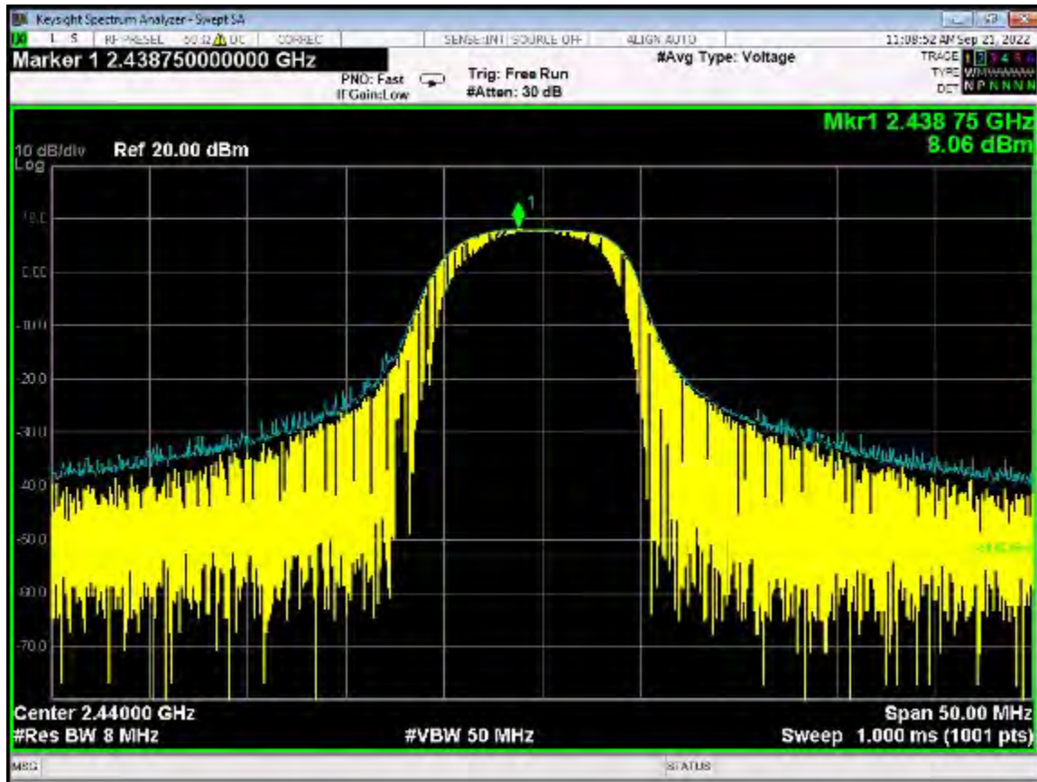
Peak Power Output – ANT 1 – 2440 MHz
