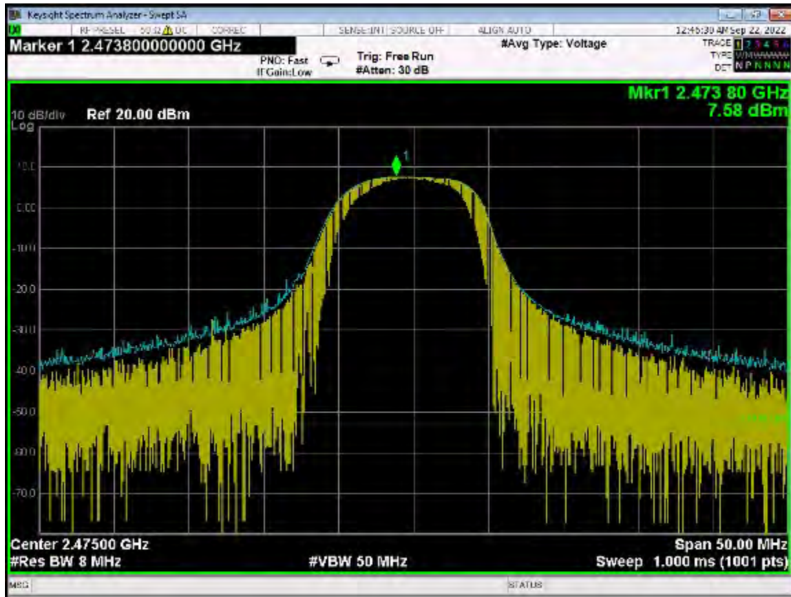
Peak Power Output – ANT 1 – 2475 MHz
