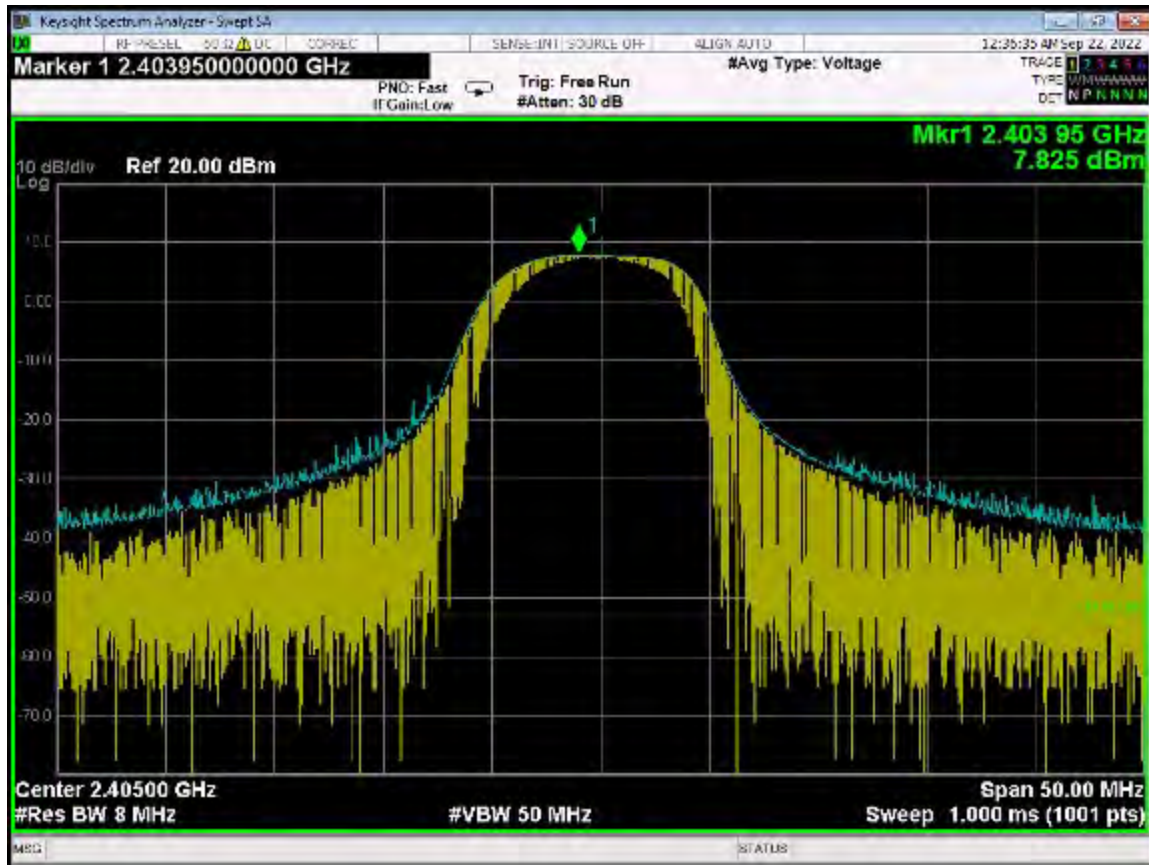
Peak Power Output – ANT 1 – 2405 MHz
