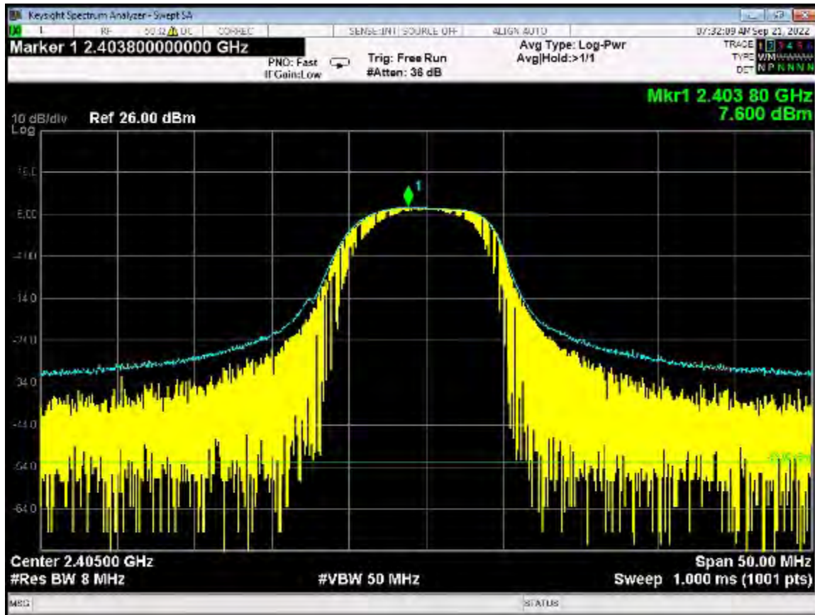
Peak Power Output – ANT 0 – 2405 MHz
