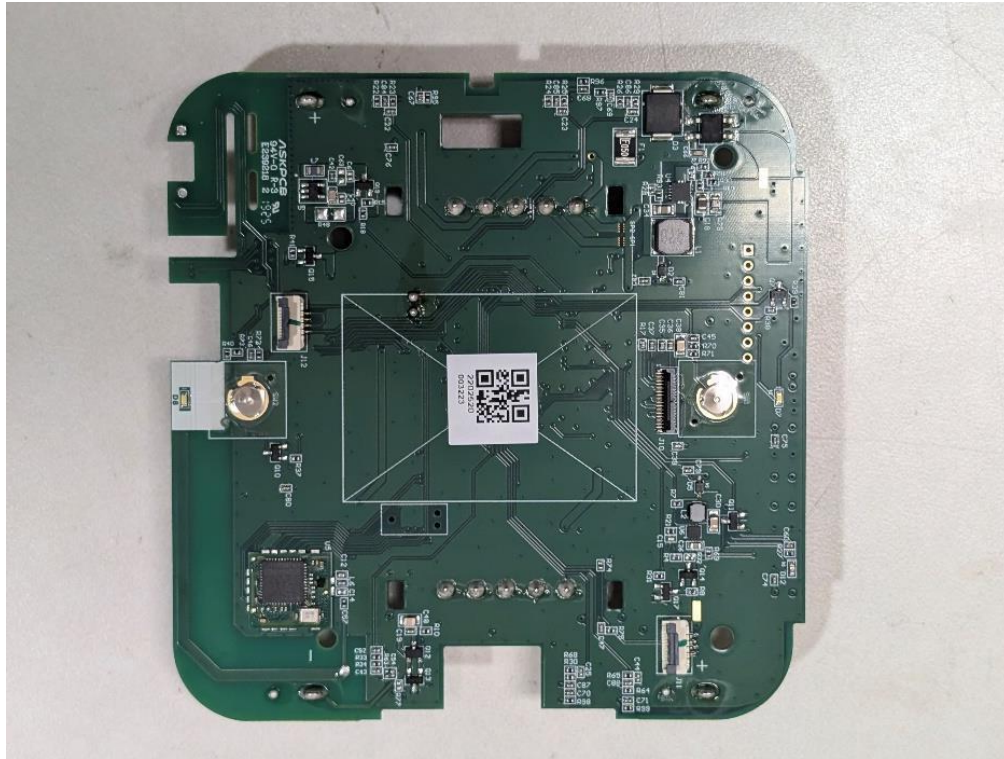
Photograph 1 –View of the Front Side of the PCB
