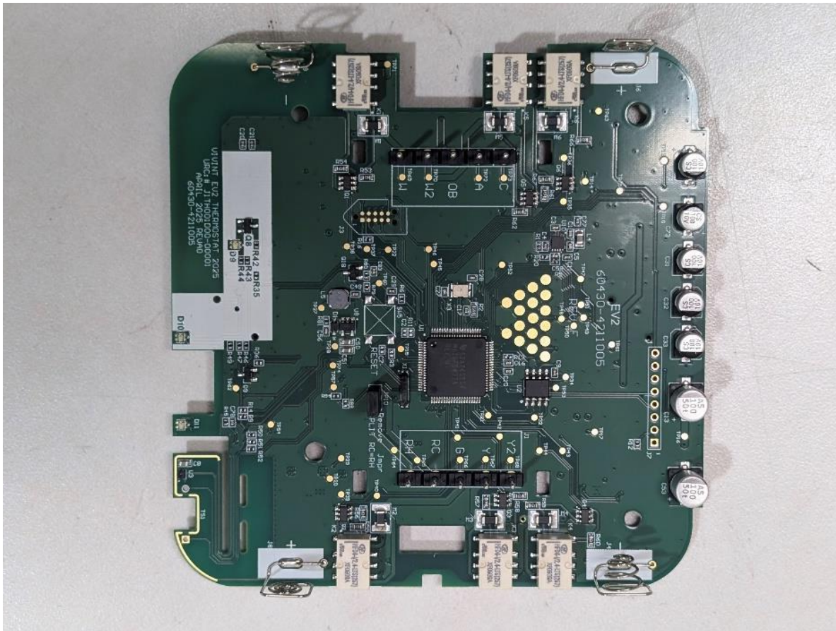
Photograph 2 – Back view of the PCB
