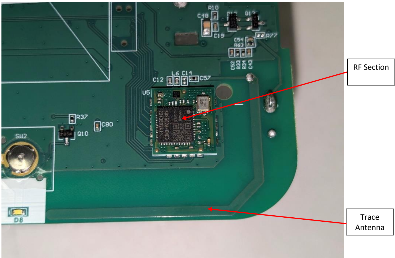
Photograph 4 – Close-up of the RF Section
