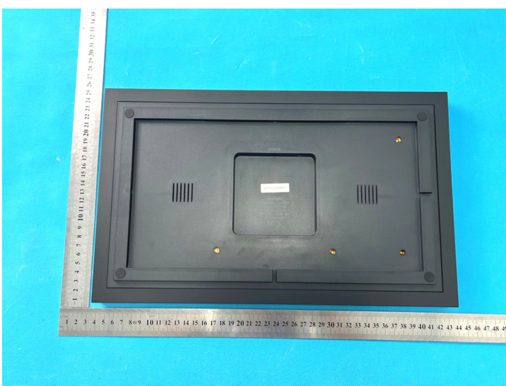
EUT View 15
