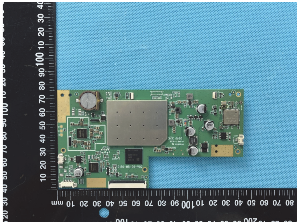
Solder Board-Component View 1
