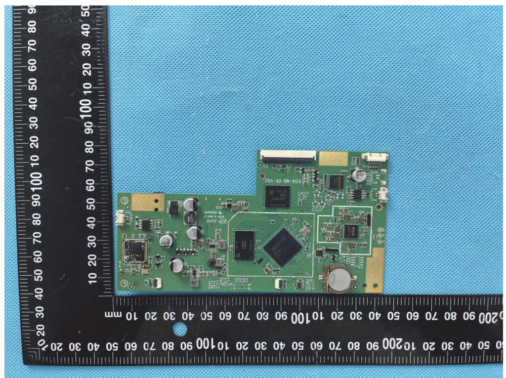
Solder Board-Component View 3
