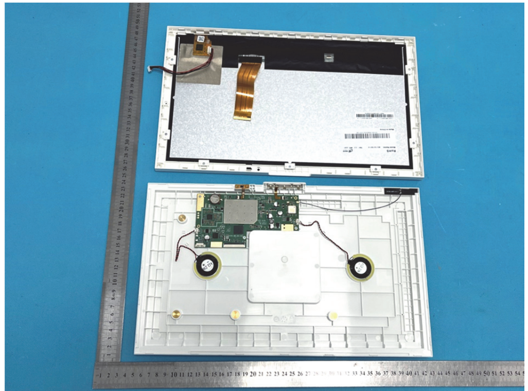
EUT Housing and Board View 1
