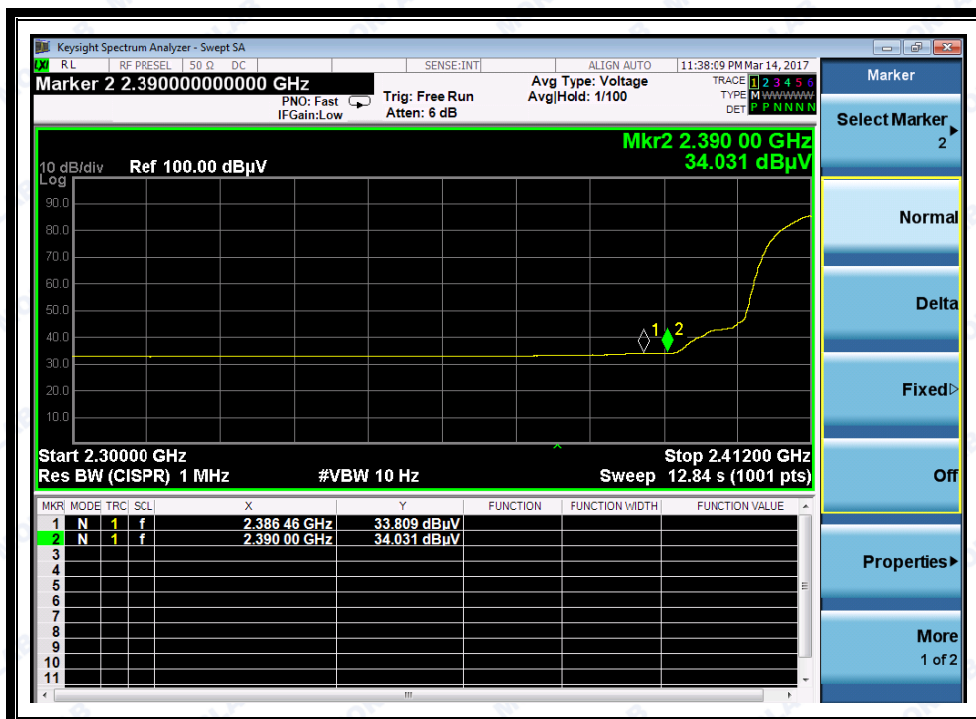
(Plot E2: Channel = 1 AVG @ 802.11n-20)
