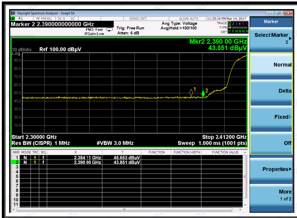
(Plot A1: Channel = 1 PEAK @ 802.11b)
