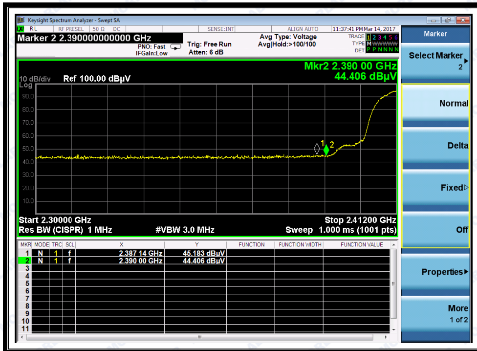
(Plot E1: Channel = 1 PEAK @ 802.11n-20)
