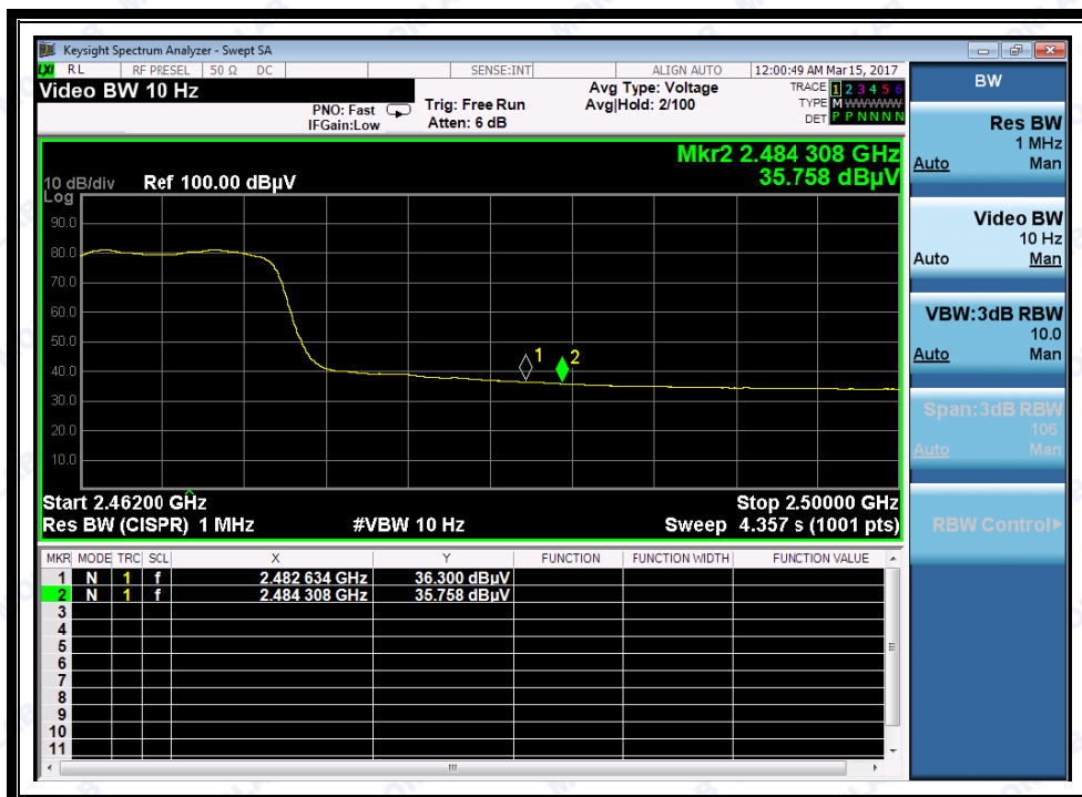
(Plot B2: Channel = 11 AVG @ 802.11b)
