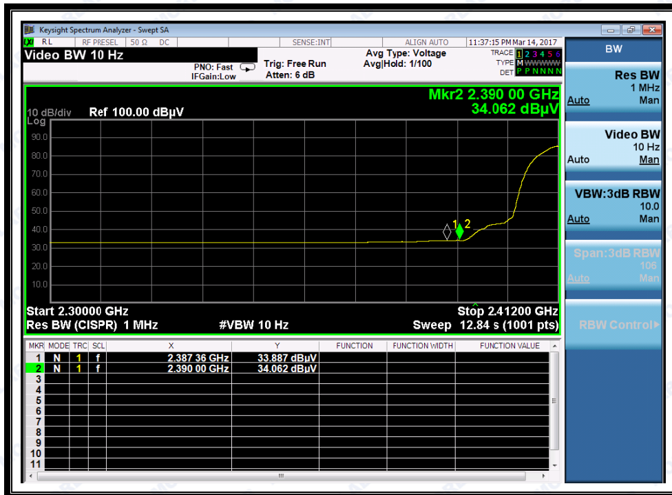
(Plot C2: Channel = 1 AVG @ 802.11g)
