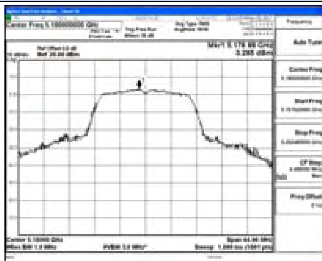
802.11a-5180MHz
