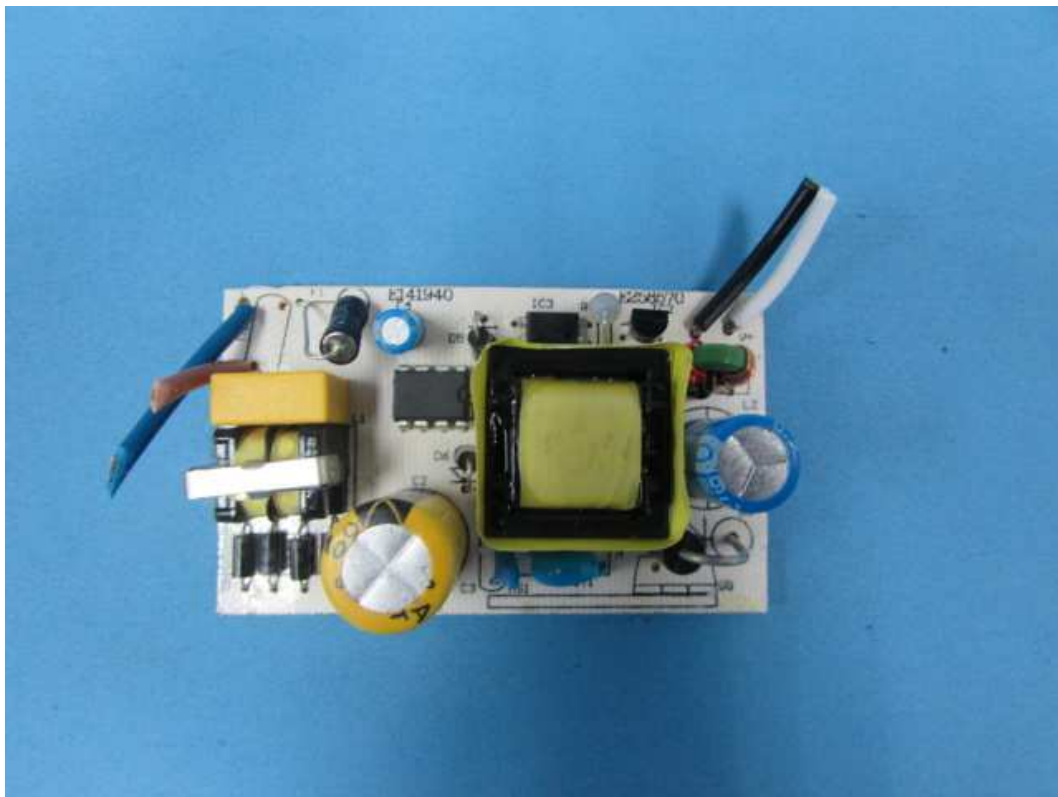
Power supply Model: MTS810-29V PCB view
