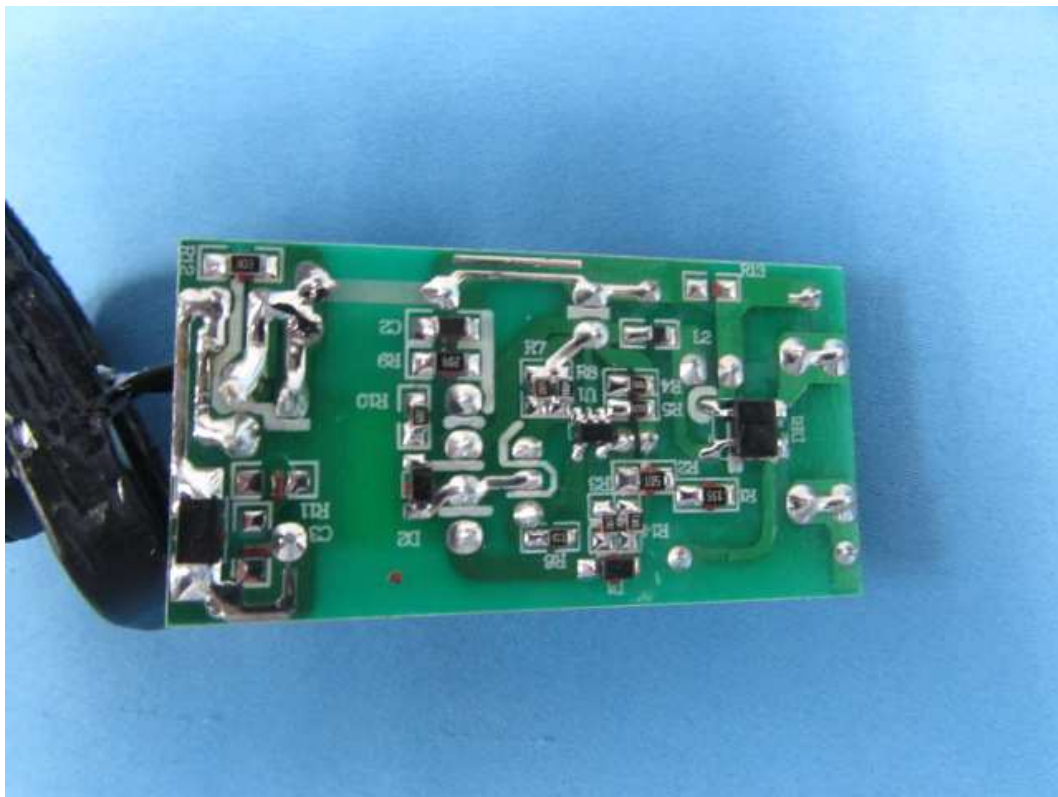
Power supply Model: TS-3W28V PCB view
