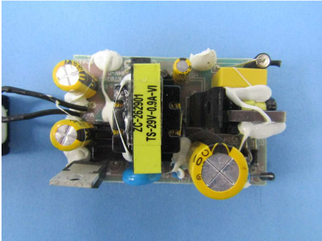
Power supply Model: TS-29V0.9A PCB view
