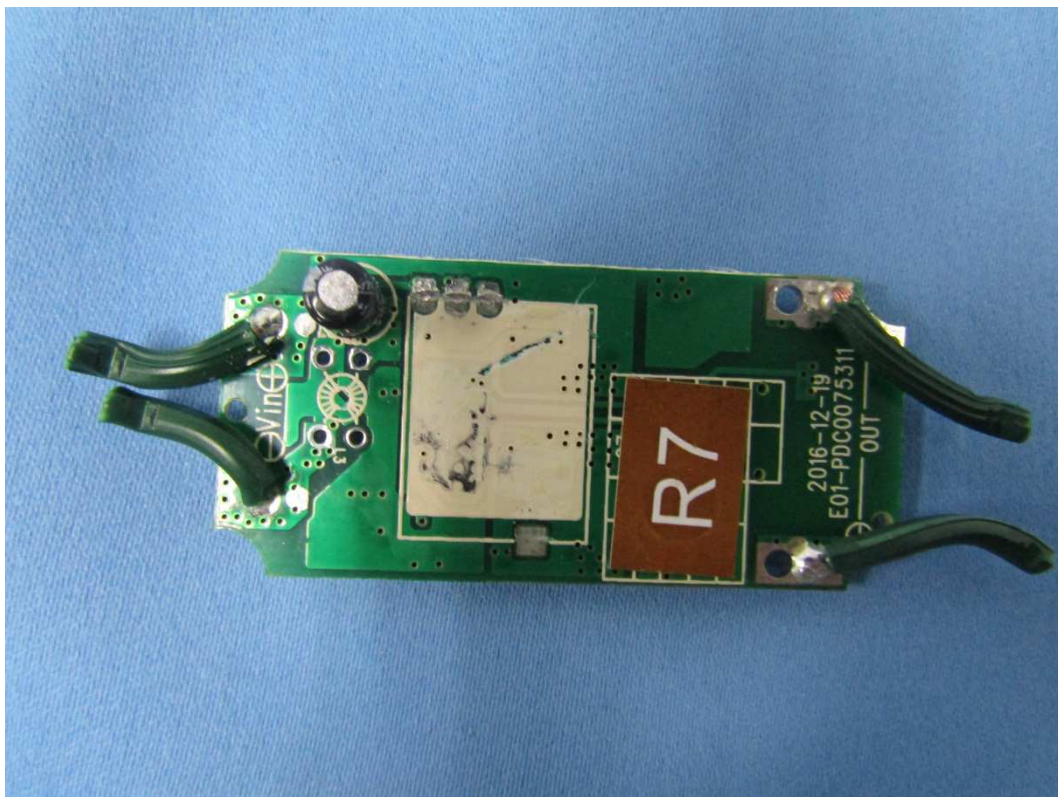
Receiver PCB view (remove the receiver module)
