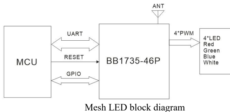
Mesh LED Sch
