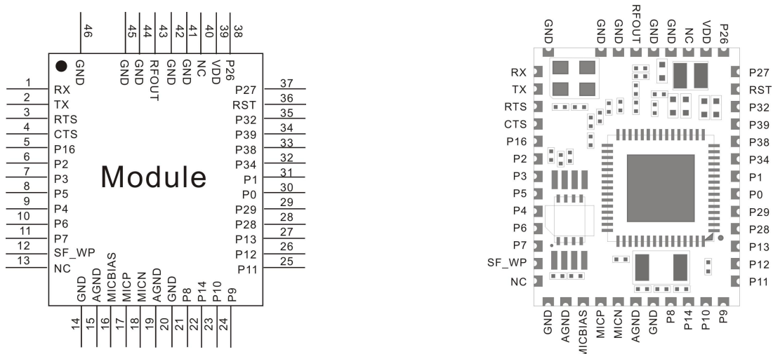
module pin assignments
