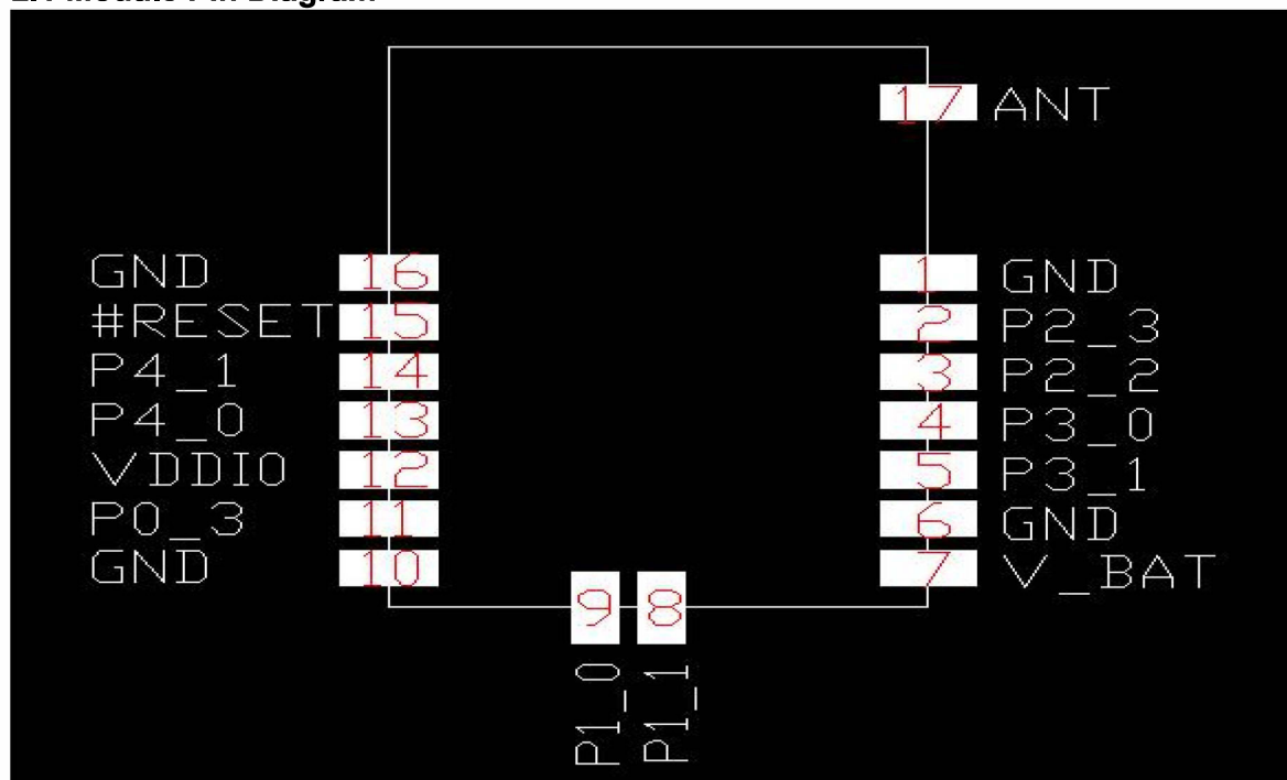
Figure 2. Pin Diagram of RB8762-17
