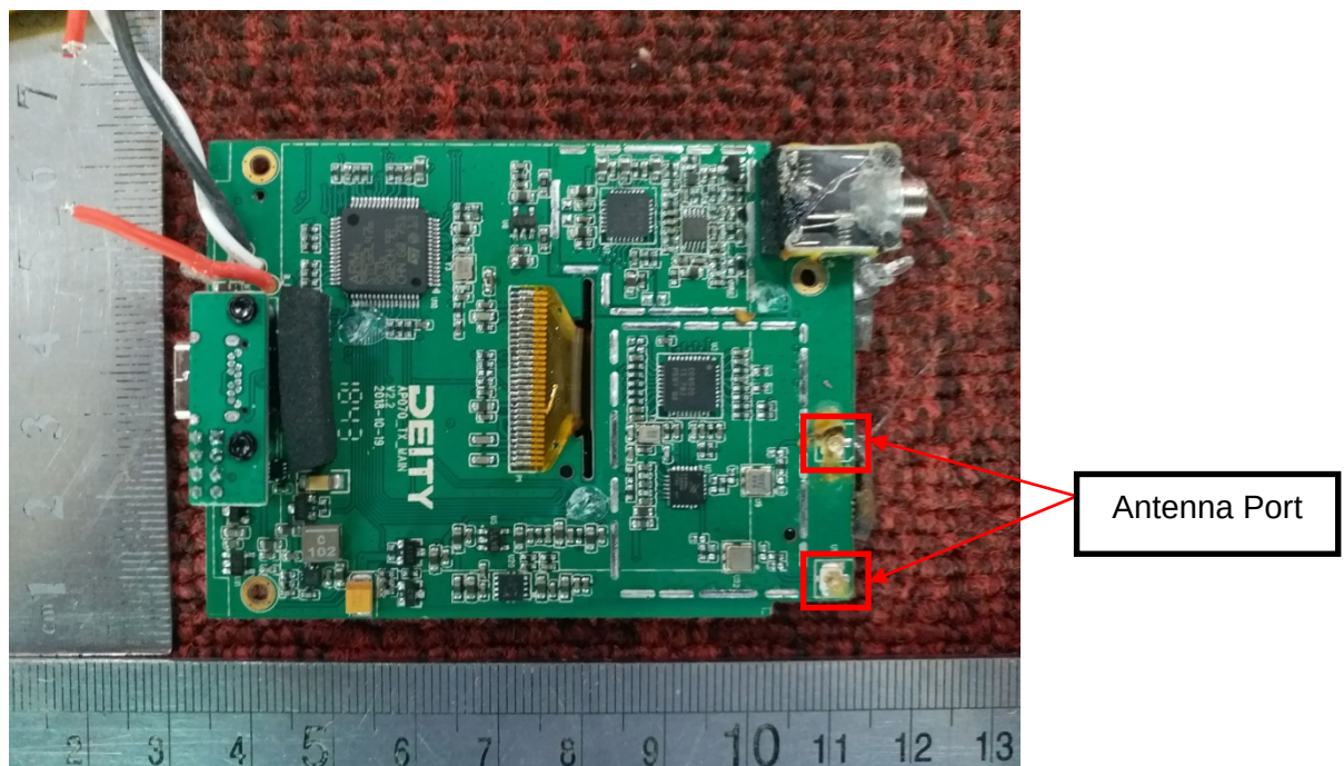
Internal photograph of EUT(TX)
