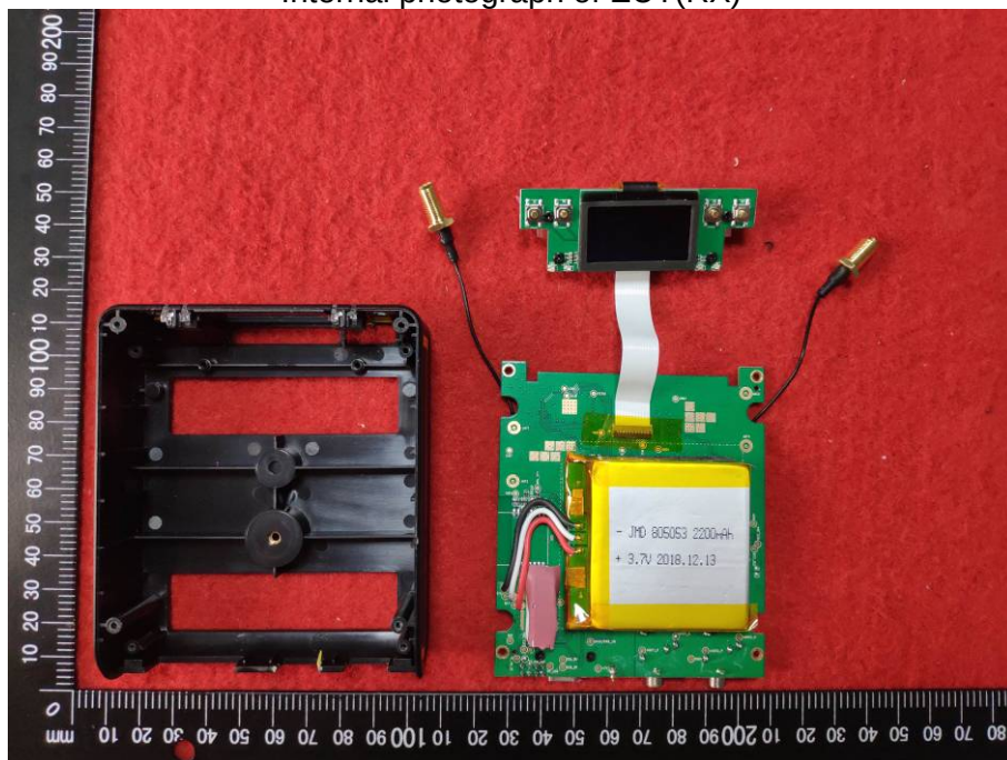
Internal photograph of EUT(RX)
