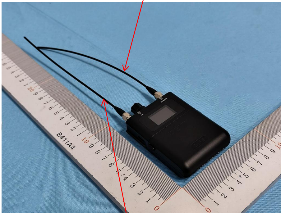
BT ANT for RF IC 1: FR3092E+ UHF RX ANT
