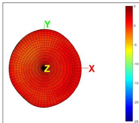
3D Radiation Gain Pattern @ 2442 MHz (unit: dBi)
