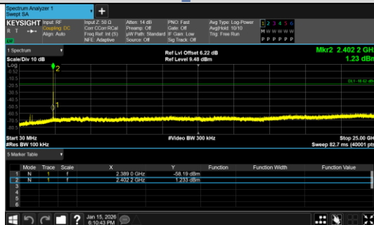
30.0 MHz - 25000.0 MHz
