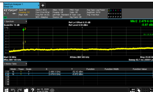
30.0 MHz - 25000.0 MHz BLE 2M_Channel 39
