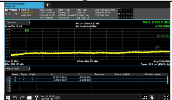
30.0 MHz - 25000.0 MHz
