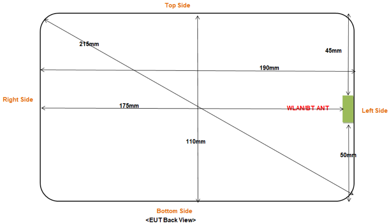
Fig 7.2 Block Diagram for EUT Antenna Position
