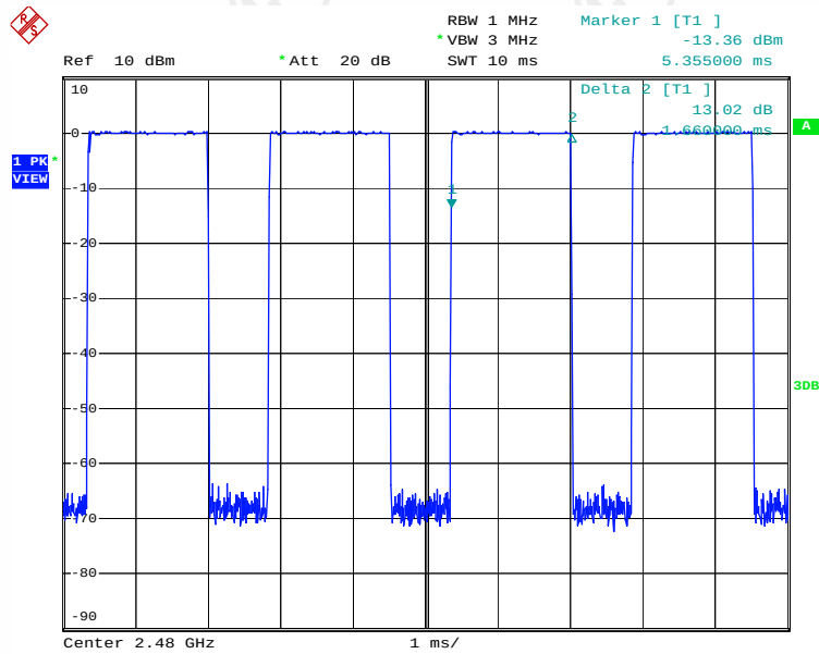
2480 MHz_DH1
