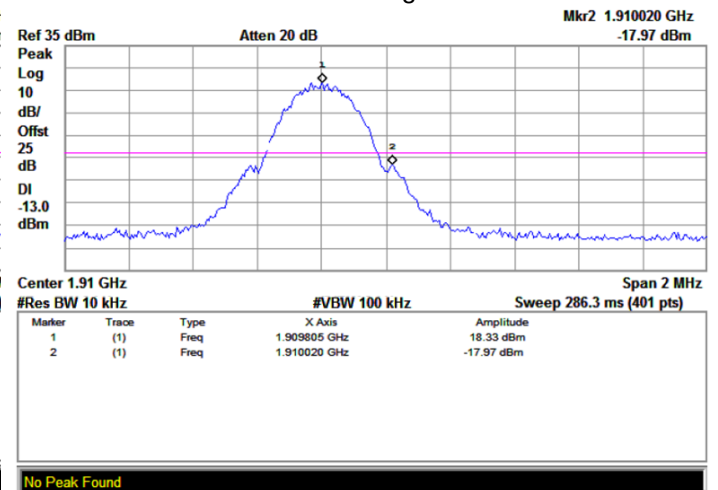
GSM 1900MHz Highest channel
