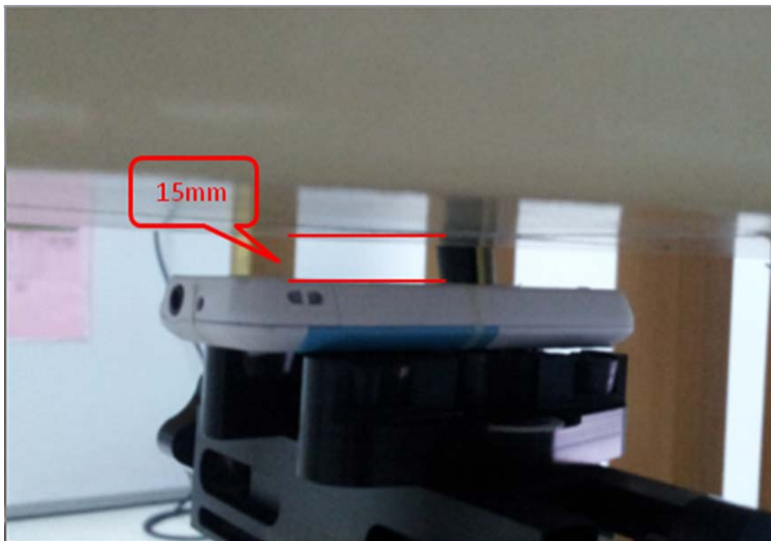
Body Worn
