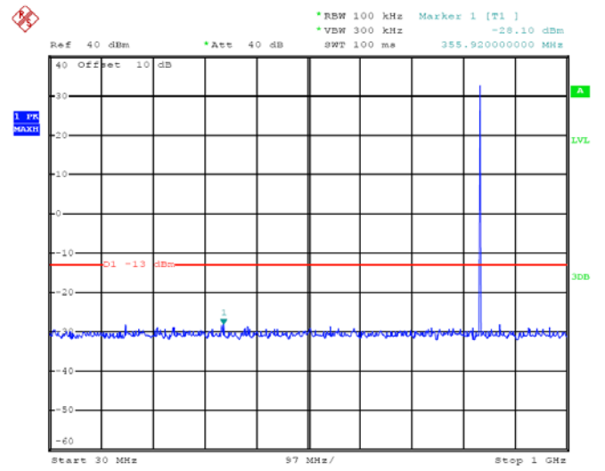
GSM 850MHz Middle channel
