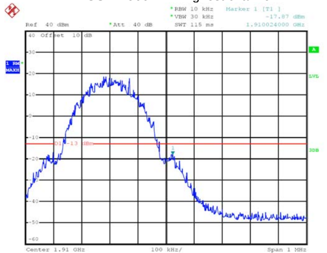
GSM 1900MHz Highest channel
