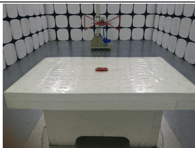
Radiated Emissions Test Setup 30MHz-1GHz
