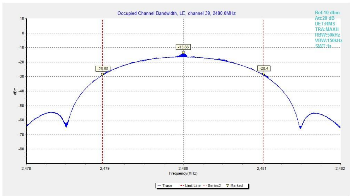
Fig.70 Occupied Bandwidth (Ch 39), 2M
