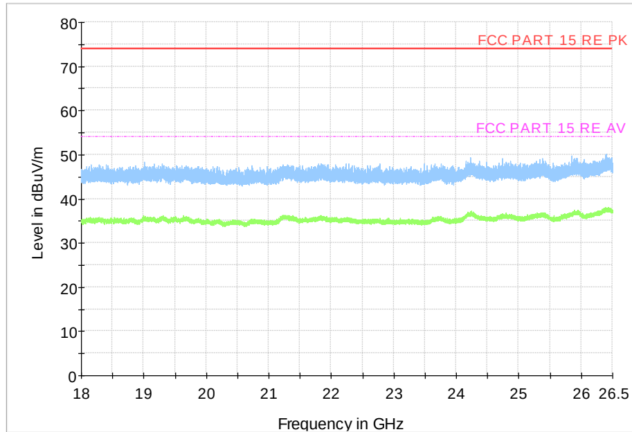
Fig.45 Radiated Spurious Emission (Ch19, 18 GHz - 26.5 GHz), 1M
