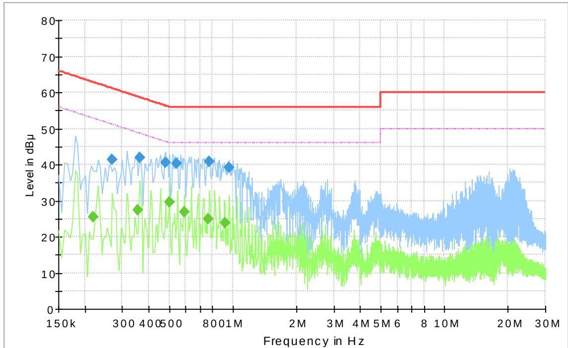
Fig.62 AC Power line Conducted Emission (Idle, AE1, 120V), 1M
