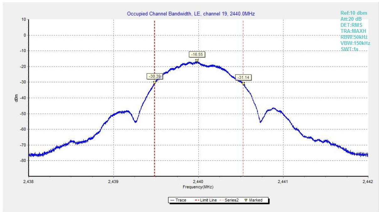
Fig.66 Occupied Bandwidth (Ch 19), 1M
