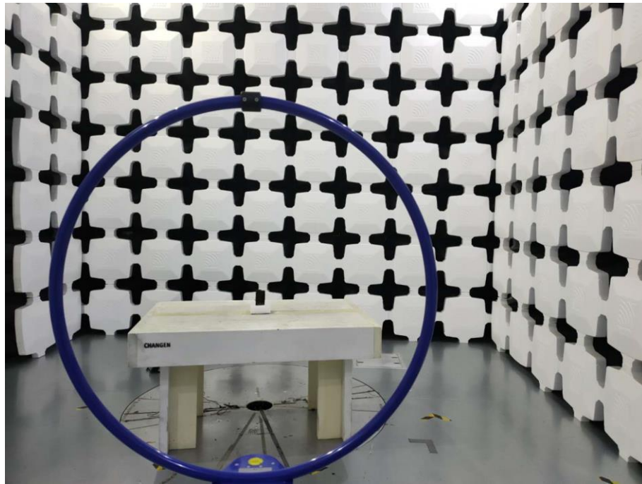
9. Radiated Emissions (Part 15C&E) (9kHz-30MHz)
