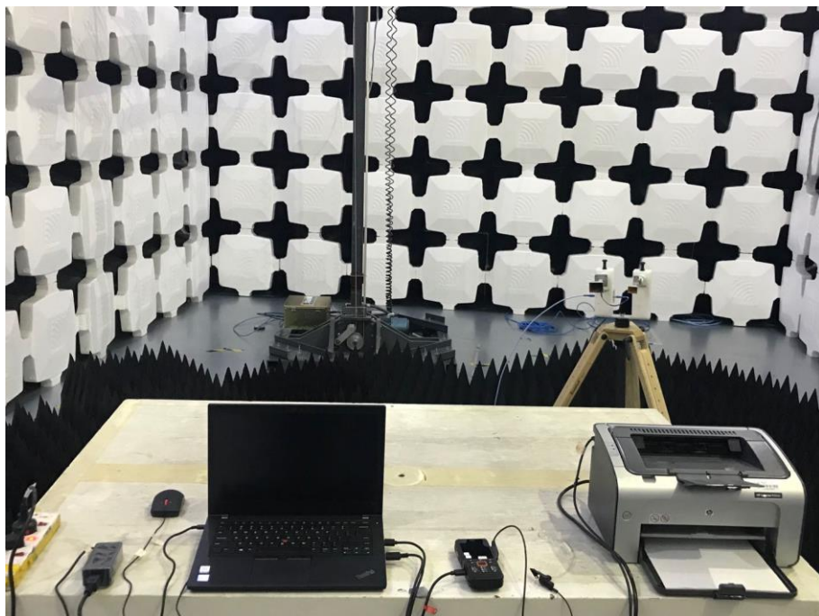
4. Radiated Emissions (Part 15B Data transfer mode)( 26.5GHz-30GHz)
