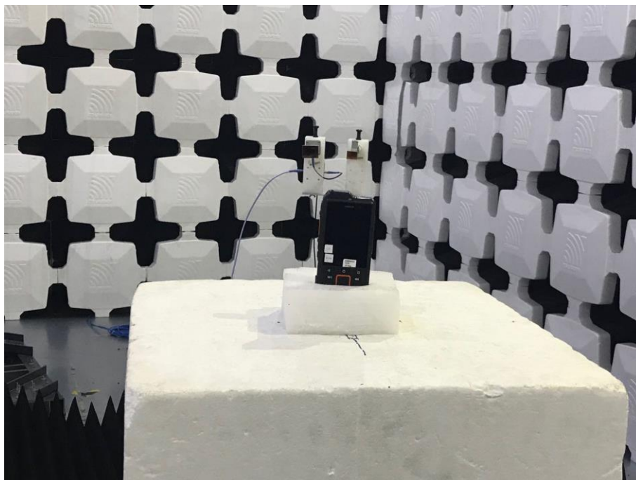
12. Radiated Emissions (Part 15C&E) (18-26.5GHz)
