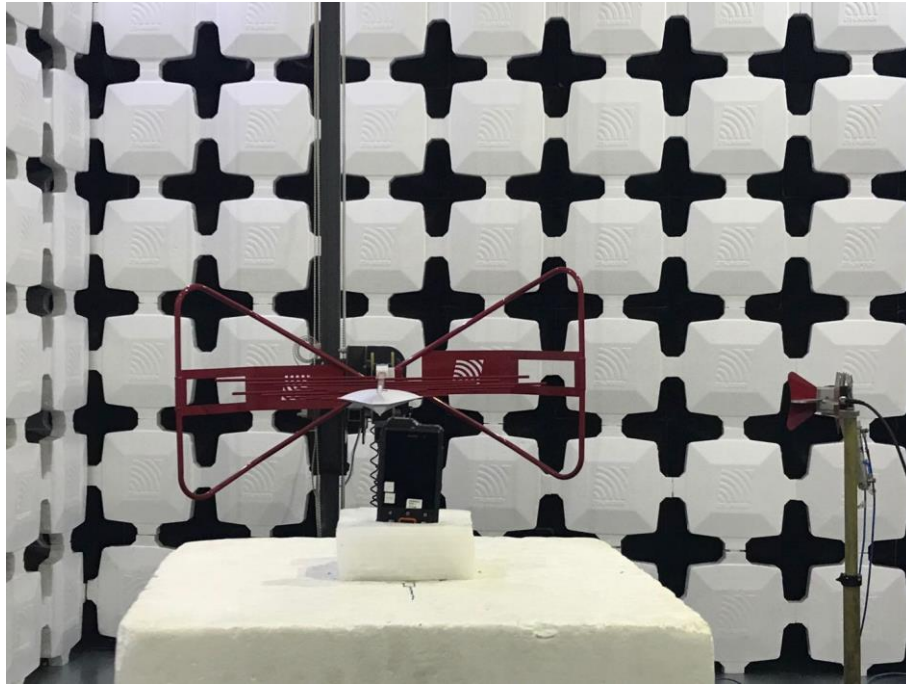
11. Radiated Emissions (Part 15C&E) (1-18GHz)
