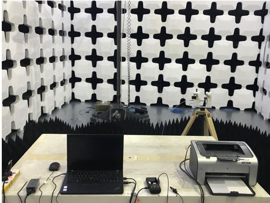
3. Radiated Emissions (Part 15B Data transfer mode)( 18GHz-26.5GHz)
