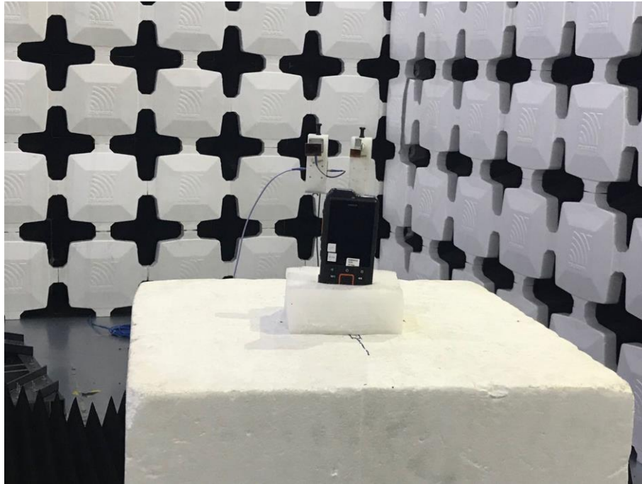
15. Radiated Emissions (Part 22/24/27/90) (18GHz-26.5GHz)
