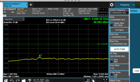
Band26_3MHz_QPSK_26775_1RB#0_1000~10000_1000~10000
