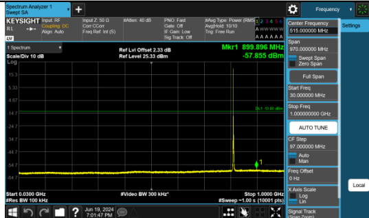
Band26_3MHz_QPSK_26705_1RB#0_30~1000_30~1000
