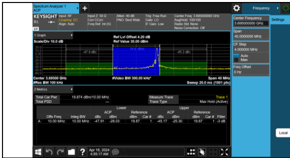
Band48-10MHz-16QAM-56690-1RB#49-PASS
