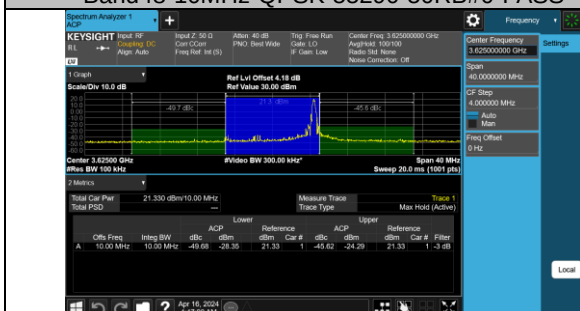
Band48-10MHz-QPSK-55990-1RB#49-PASS
