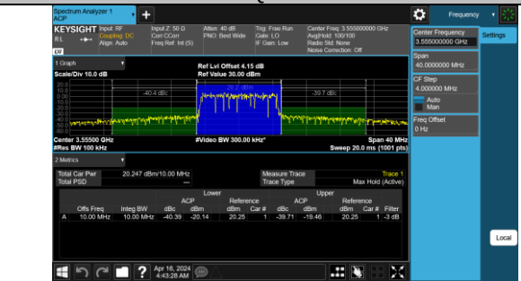
Band48-10MHz-16QAM-55290-50RB#0-PASS
