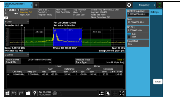
Band48-5MHz-16QAM-56715-1RB#0-PASS
