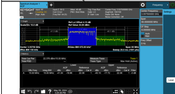
Band48-15MHz-QPSK-55315-75RB#0-PASS
