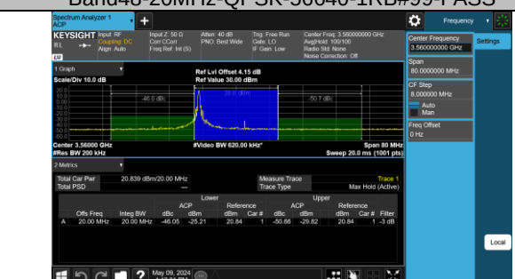
Band48-20MHz-16QAM-55340-1RB#0-PASS
