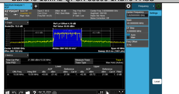
Band48-10MHz-QPSK-55990-50RB#0-PASS
