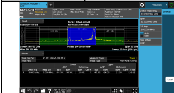
Band48-5MHz-16QAM-56715-1RB#24-PASS
