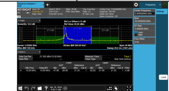
Band48-10MHz-16QAM-55290-1RB#0-PASS
