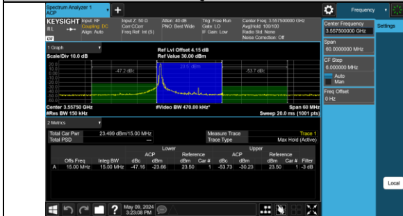
Band48-15MHz-QPSK-55315-1RB#0-PASS
