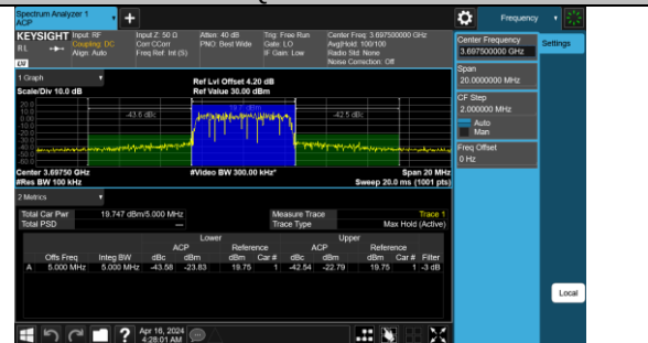
Band48-5MHz-16QAM-56715-25RB#0-PASS
