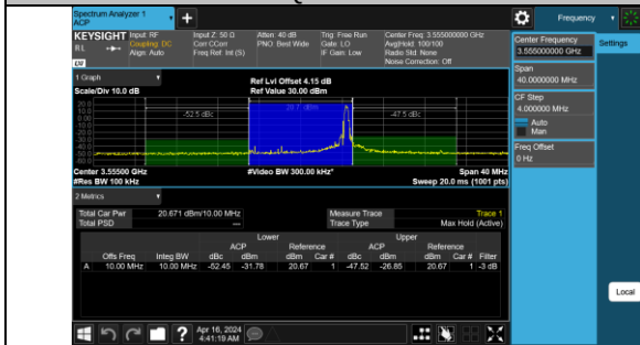
Band48-10MHz-16QAM-55290-1RB#49-PASS
