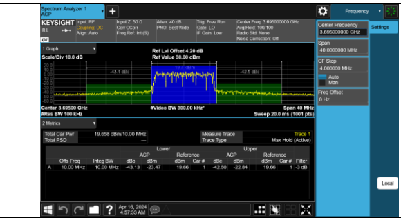
Band48-10MHz-16QAM-56690-50RB#0-PASS
