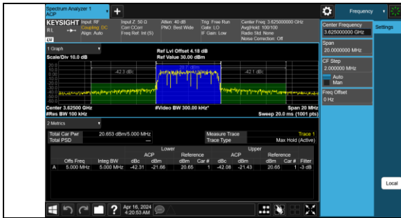
Band48-5MHz-16QAM-55990-25RB#0-PASS
