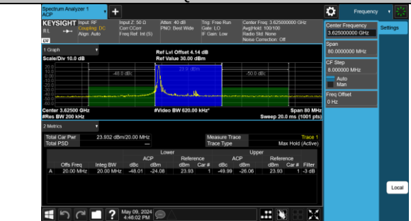
Band48-20MHz-QPSK-55990-1RB#0-PASS
