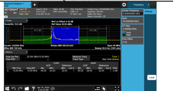
Band48-10MHz-QPSK-55990-1RB#0-PASS
