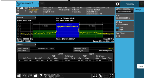
Band48-20MHz-QPSK-55340-100RB#0-PASS
