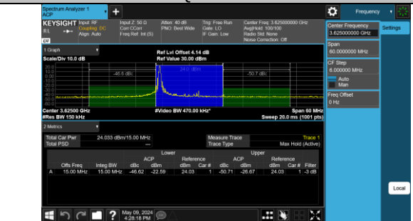
Band48-15MHz-QPSK-55990-1RB#0-PASS
