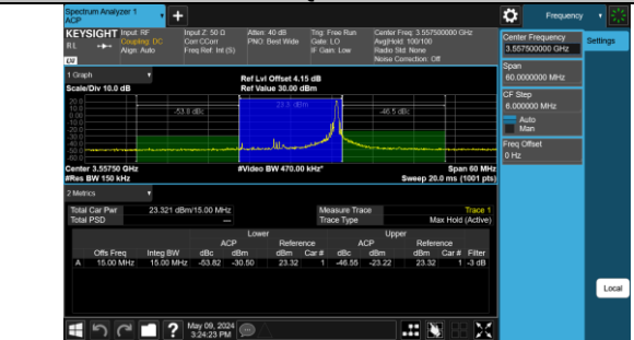
Band48-15MHz-QPSK-55315-1RB#74-PASS
