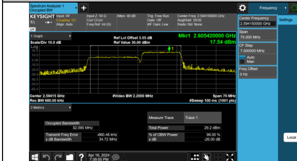
41-41-20MHz-15MHz-16QAM-16QAM-40546-40717-100 RB#0-75RB#0-PASS
