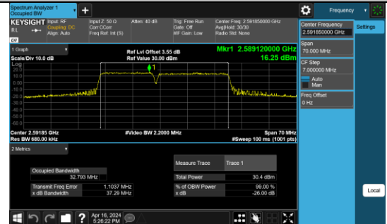
41-41-15MHz-20MHz-QPSK-QPSK-40523-40694-75RB #0-100RB#0-PASS
