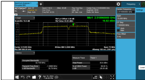
41-41-20MHz-15MHz-QPSK-QPSK-39750-39921-100R B#0-75RB#0-PASS
