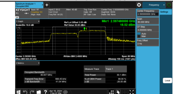
41-41-20MHz-20MHz-QPSK-QPSK-40521-40719-100R B#0-100RB#0-PASS
