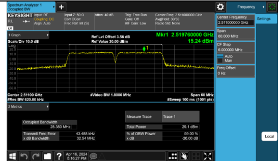
41-41-15MHz-15MHz-16QAM-16QAM-39725-39875-75RB #0-75RB#0-PASS
