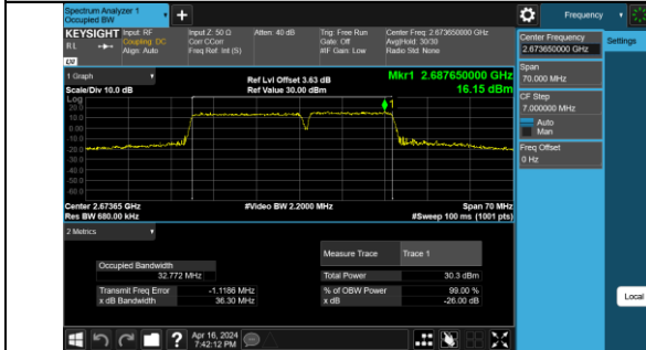
41-41-20MHz-15MHz-QPSK-QPSK-41341-41512-100R B#0-75RB#0-PASS
