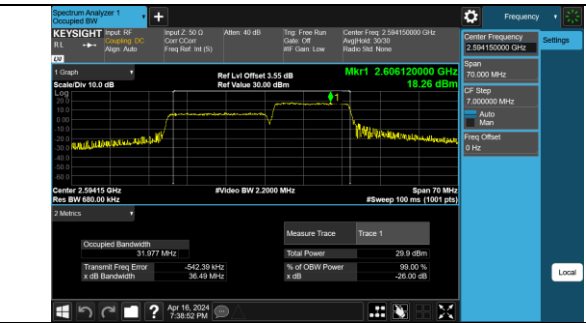
41-41-20MHz-15MHz-QPSK-QPSK-40546-40717-100R B#0-75RB#0-PASS
