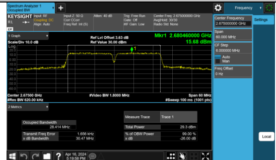
41-41-15MHz-15MHz-16QAM-16QAM-41365-41515-75RB #0-75RB#0-PASS
