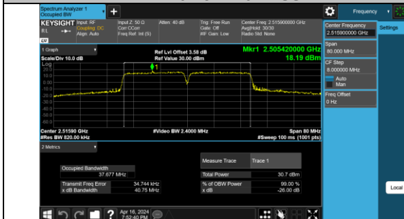
41-41-20MHz-20MHz-QPSK-QPSK-39750-39948-100R B#0-100RB#0-PASS
