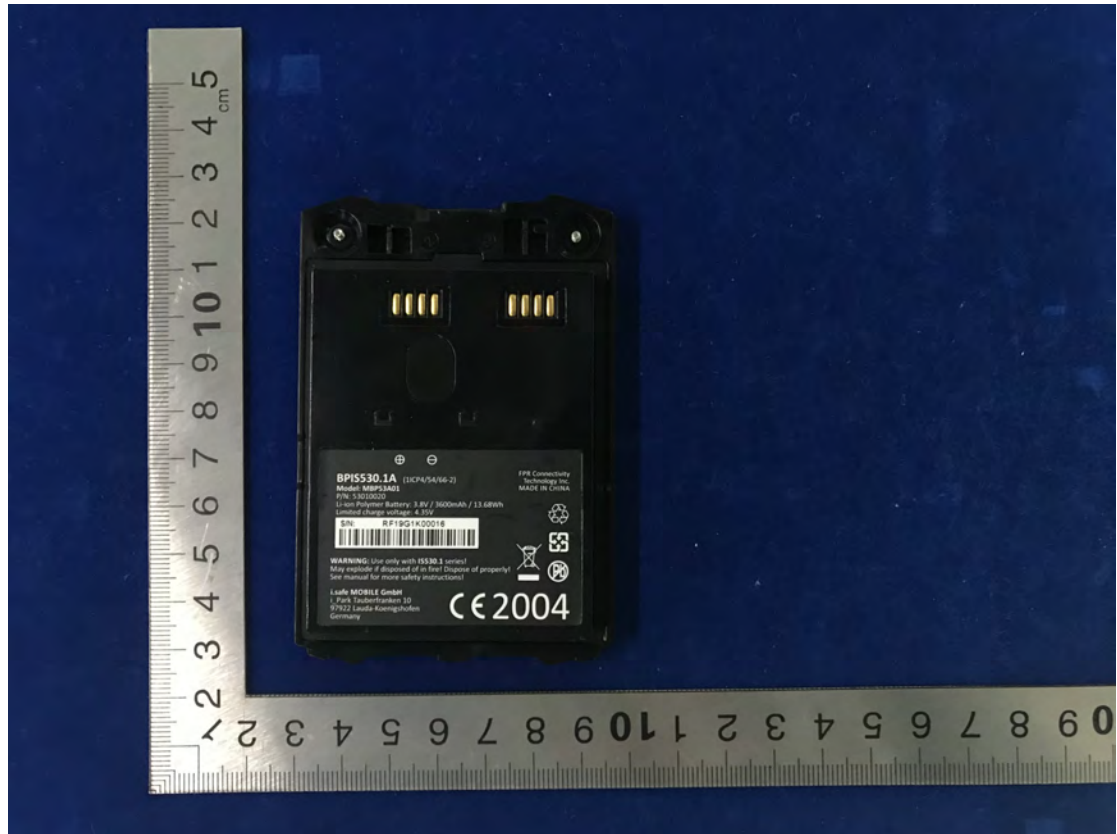
Battery-1
