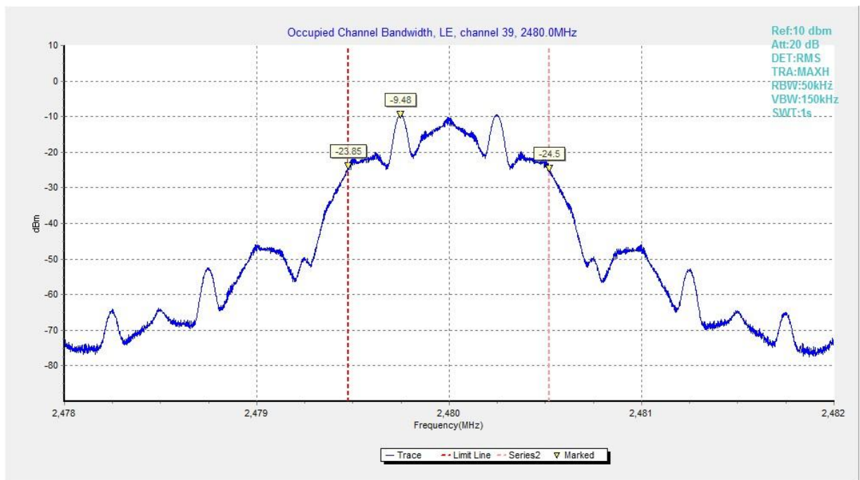
Fig.120 Occupied Bandwidth (Ch 39), LE Coded (S=8)
