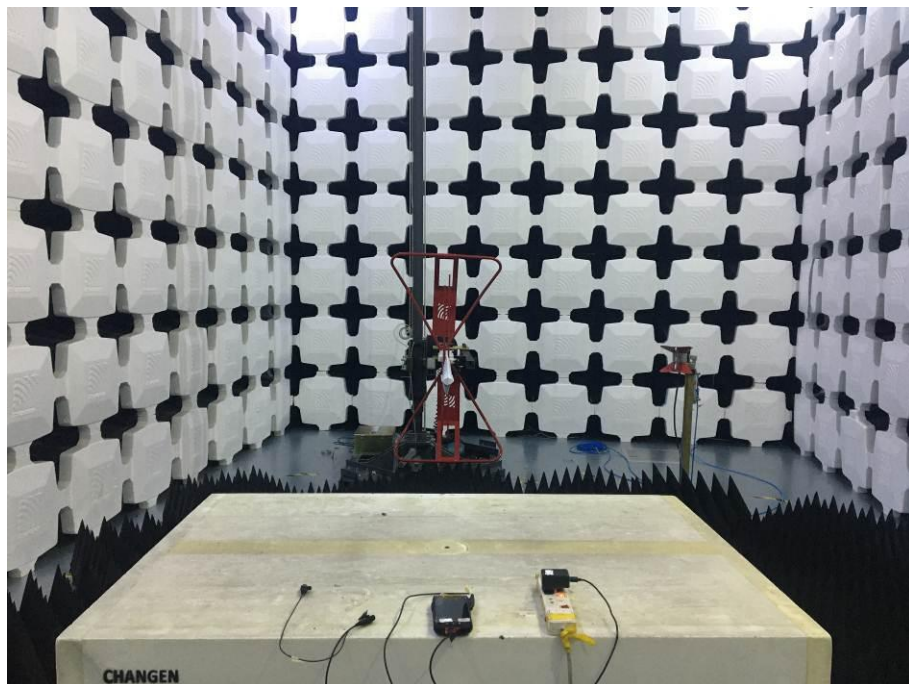
8. Radiated Emissions (Part 15B Charging mode Type C Wire + Headset) (1GHz-18GHz)
