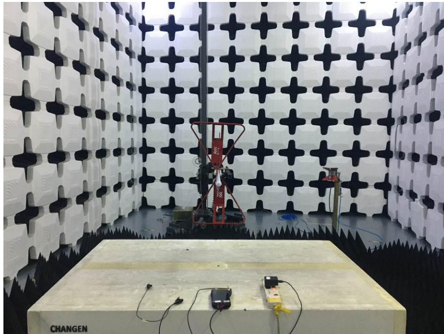
7. Radiated Emissions (Part 15B Charging mode Magnetic wire+Headset) (1GHz-18GHz)
