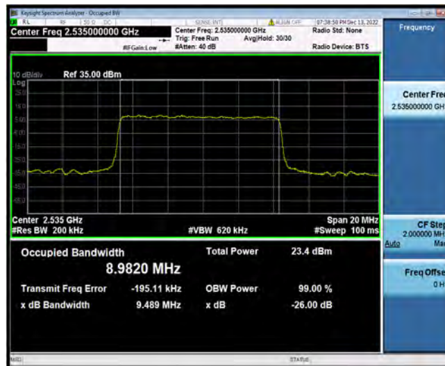
N7-10MHz-64QAM-507000-50RB#0
