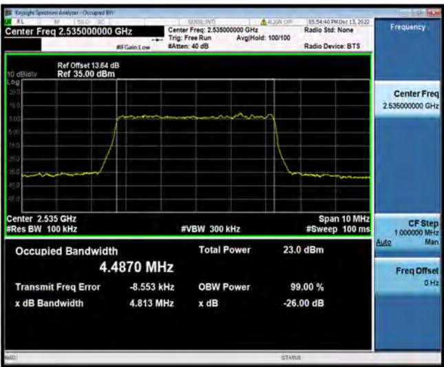
N7-5MHz-64QAM-507000-25RB#0
