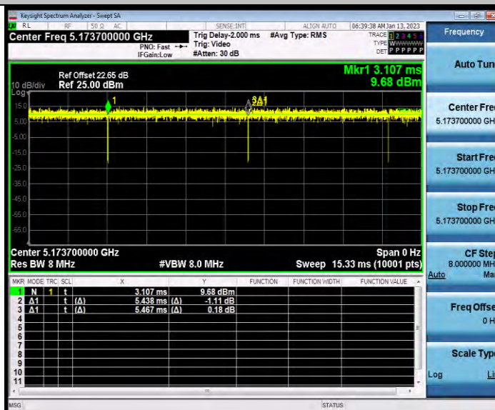
11AX20_RU_Ant2_5180_242Tone_RU61
