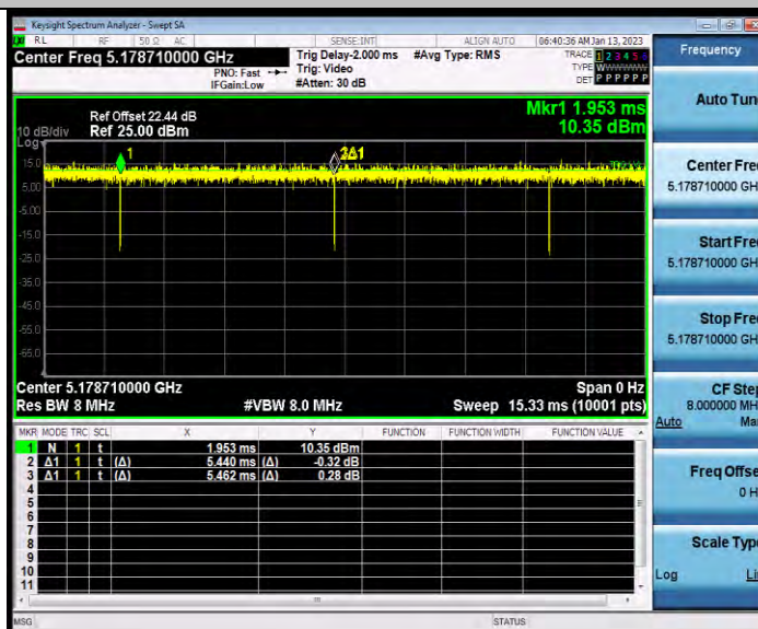
11AX20_RU_Ant1_5200_242Tone_RU61
