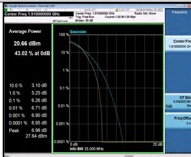
Band25-10MHz-64QAM-26640-50RB#0
