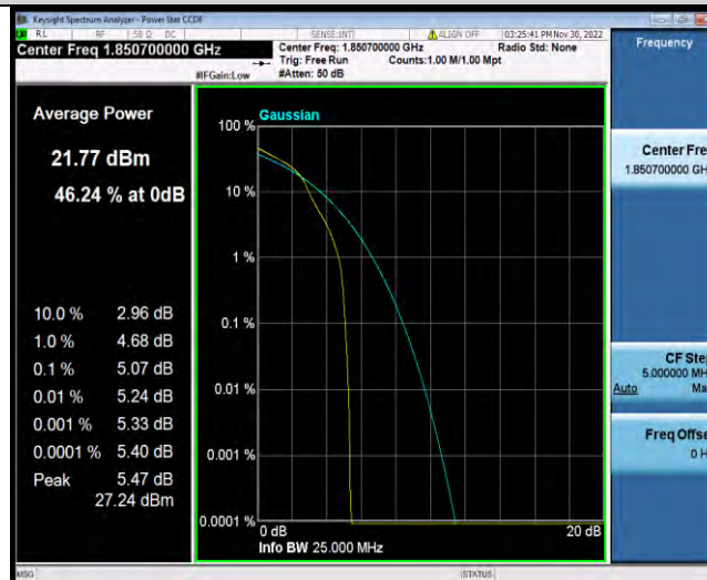
Band25-1.4MHz-16QAM-26047-6RB#0
