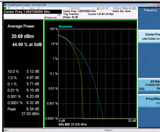
Band25-1.4MHz-16QAM-26365-1RB#0
