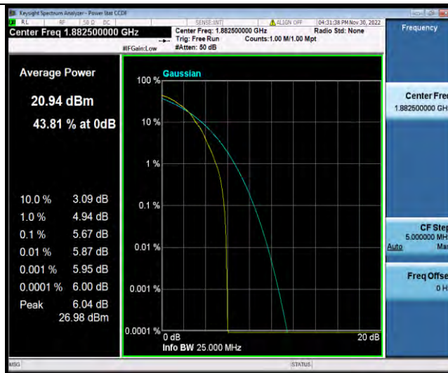
Band25-3MHz-64QAM-26365-15RB#0
