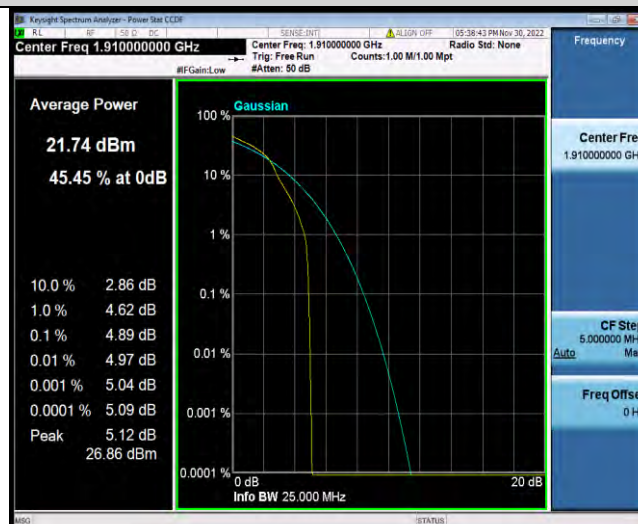
Band25-10MHz-16QAM-26640-50RB#0
