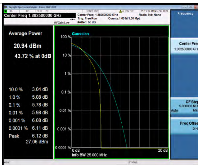
Band25-5MHz-64QAM-26365-25RB#0
