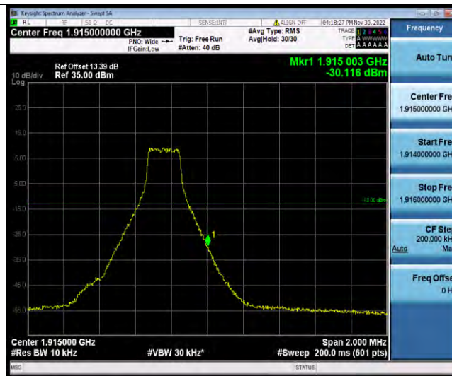
Band25-3MHz-64QAM-26675-15RB#0
