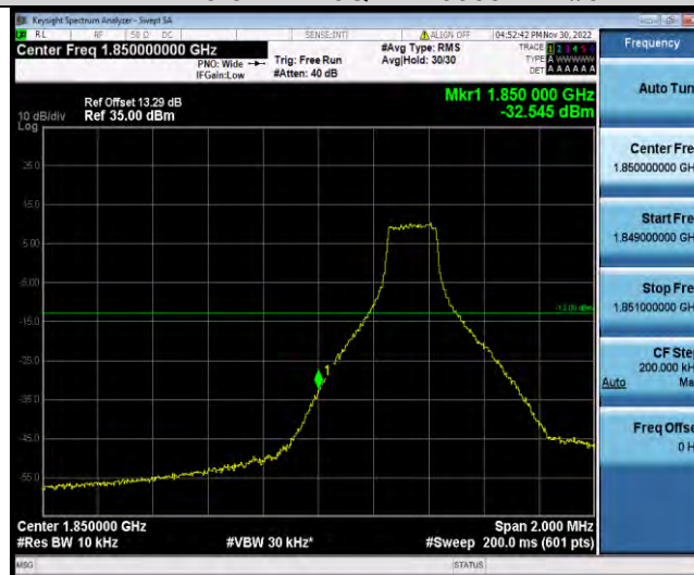
Band25-5MHz-16QAM-26065-1RB#24
