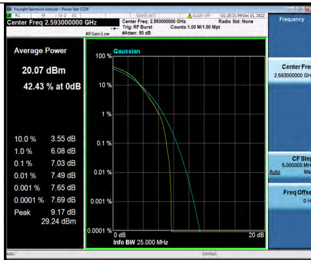
Band41-20MHz-64QAM-40620-100RB#0
