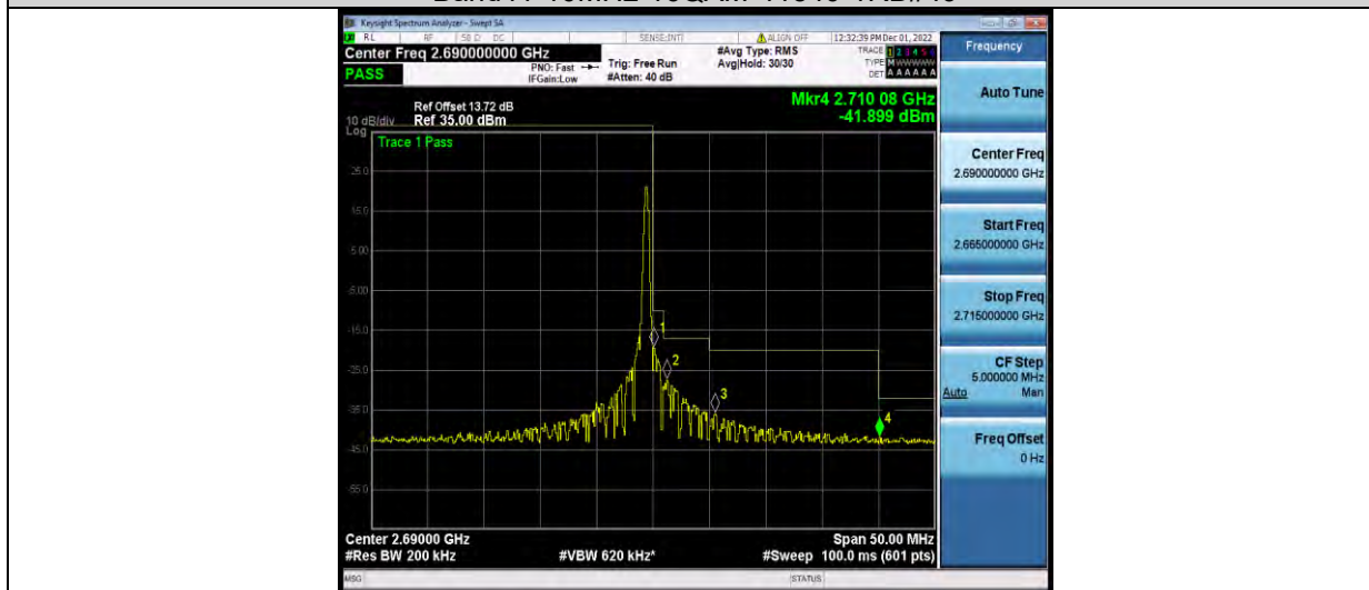
Band41-10MHz-16QAM-41540-50RB#0
