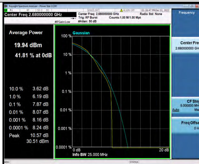
Band41-20MHz-64QAM-41490-100RB#0
