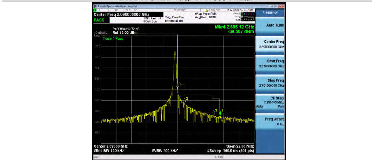
Band41-5MHz-16QAM-41565-25RB#0
