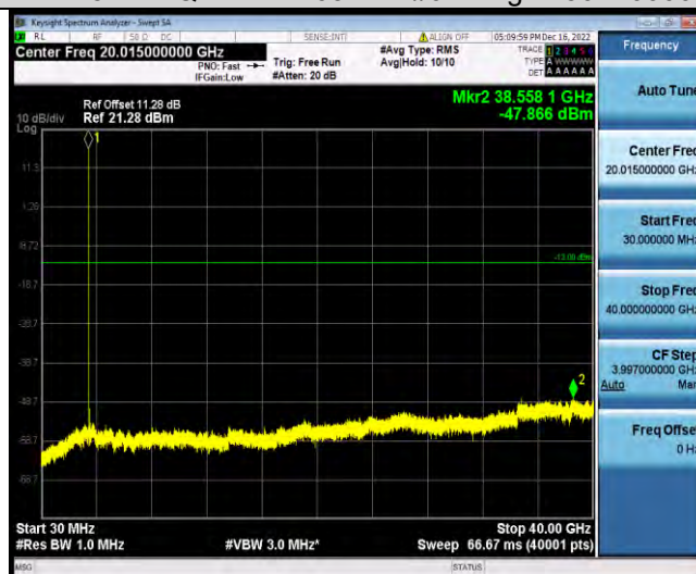
Band42-15MHz-QPSK-42590-1RB#0-Range1:30~40000MHz
