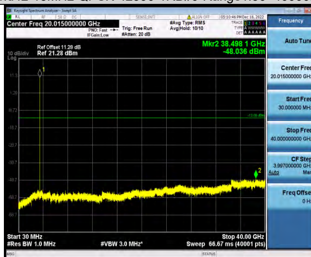
Band42-15MHz-QPSK-43015-1RB#0-Range1:30~40000MHz
