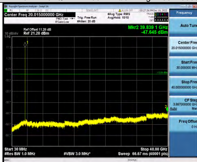
Band42-20MHz-64QAM-42590-1RB#0-Range1:30~40000MHz
