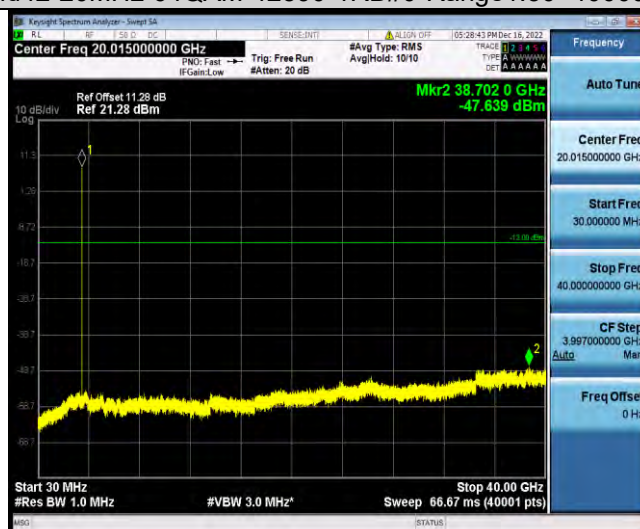
Band42-20MHz-64QAM-42990-1RB#0-Range1:30~40000MHz
