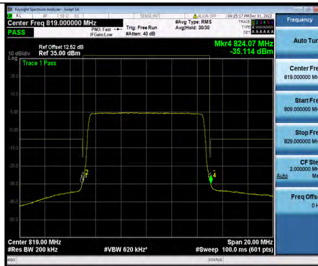
Band26-10MHz-64QAM-26740-1RB#0
