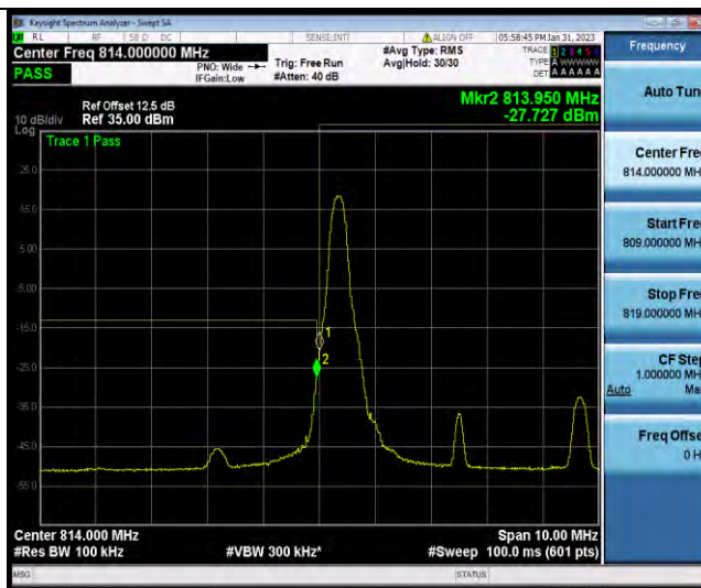
Band26-5MHz-64QAM-26715-25RB#0
