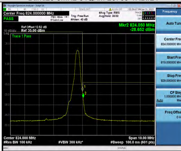
Band26-5MHz-64QAM-26765-25RB#0
