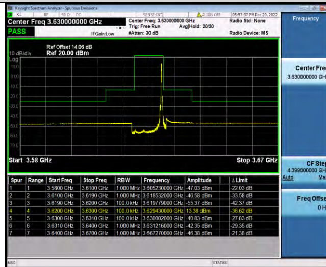
Band48-10MHz-QPSK-55990-50RB#0
