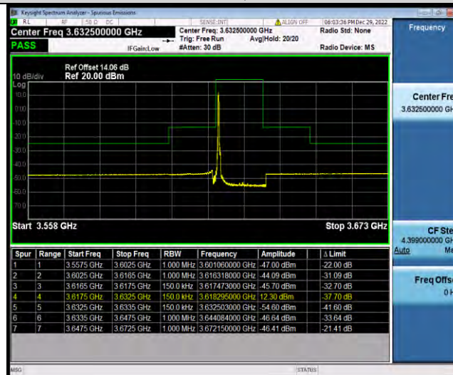
Band48-15MHz-64QAM-55990-1RB#74
