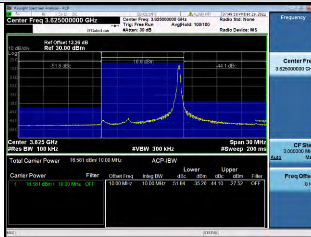
Band48-10MHz-QPSK-55990-50RB#0
