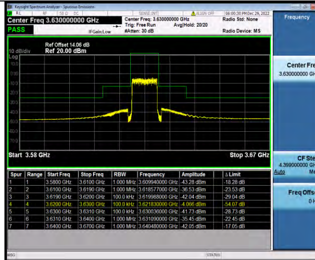
Band48-10MHz-16QAM-56690-1RB#0
