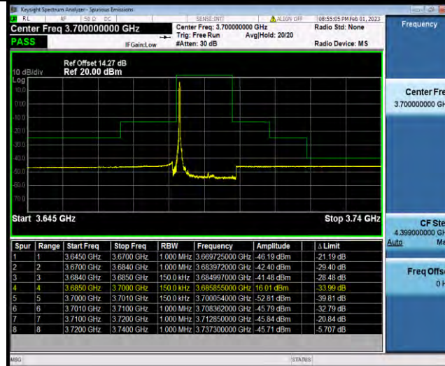
Band48-15MHz-QPSK-56665-1RB#74
