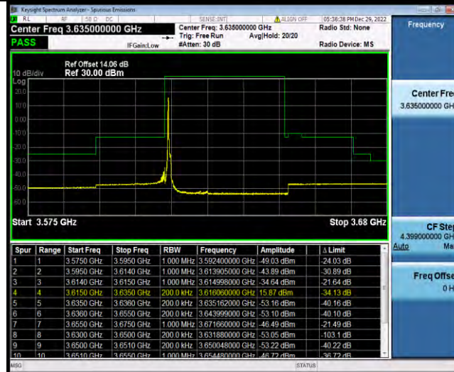
Band48-20MHz-QPSK-55990-1RB#99
