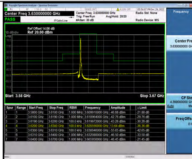
Band48-10MHz-16QAM-55990-1RB#49
