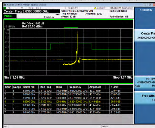
Band48-10MHz-16QAM-55990-50RB#0
