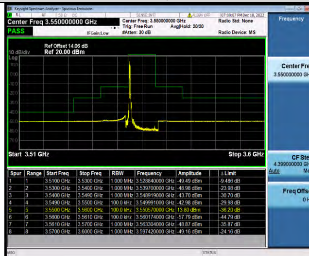
Band48-10MHz-16QAM-55290-1RB#49
