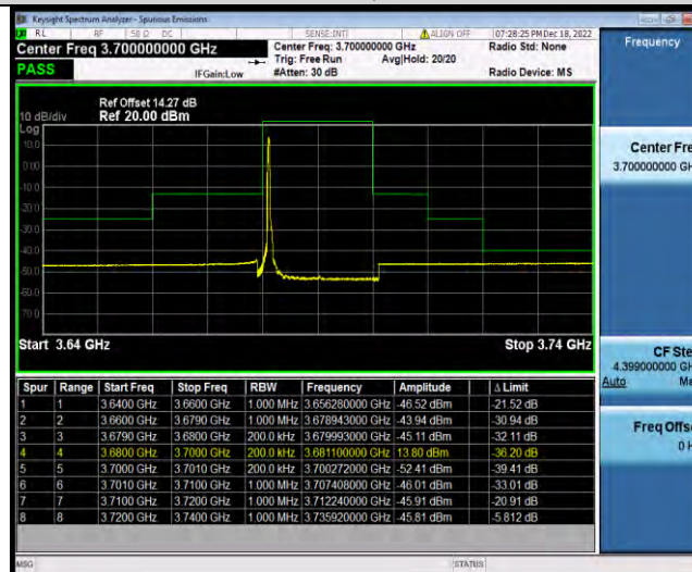
Band48-20MHz-64QAM-56640-1RB#99
