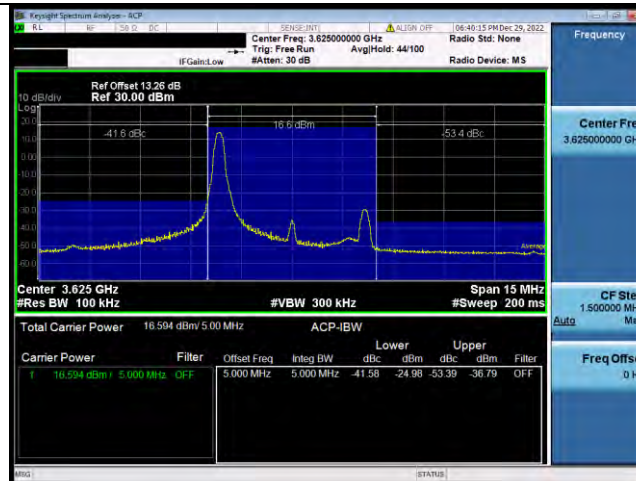
Band48-5MHz-QPSK-55990-1RB#24
