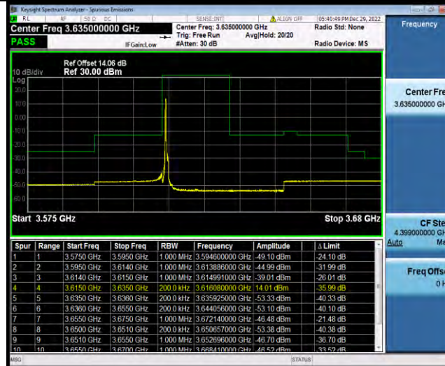
Band48-20MHz-64QAM-55990-1RB#99
