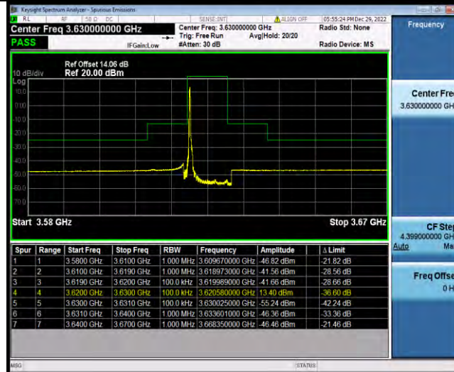
Band48-10MHz-QPSK-55990-1RB#49
