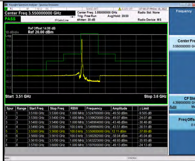
Band48-10MHz-64QAM-55290-1RB#49
