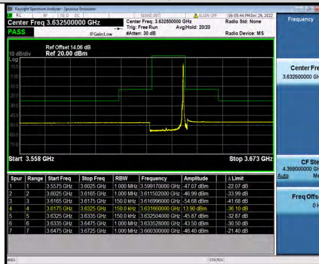
Band48-15MHz-64QAM-55990-75RB#0
