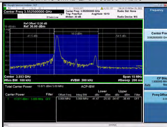
Band48-5MHz-QPSK-55265-1RB#24
