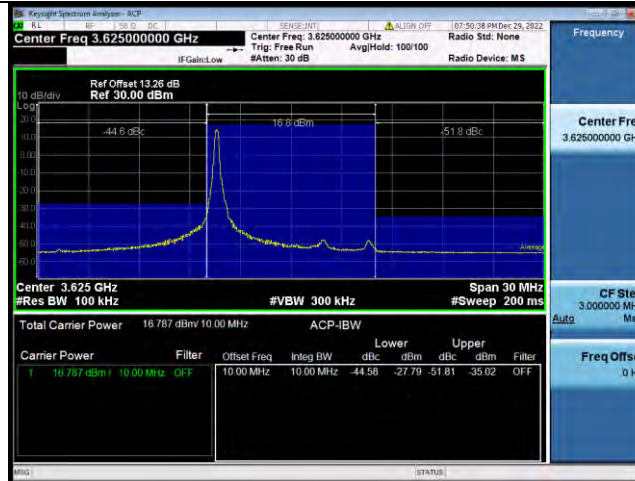
Band48-10MHz-QPSK-55990-1RB#49
