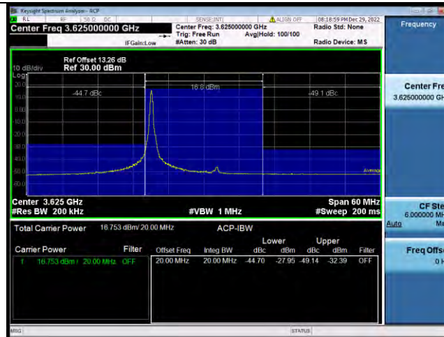
Band48-20MHz-QPSK-55990-1RB#99
