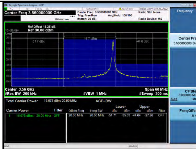
Band48-20MHz-QPSK-55340-100RB#0
