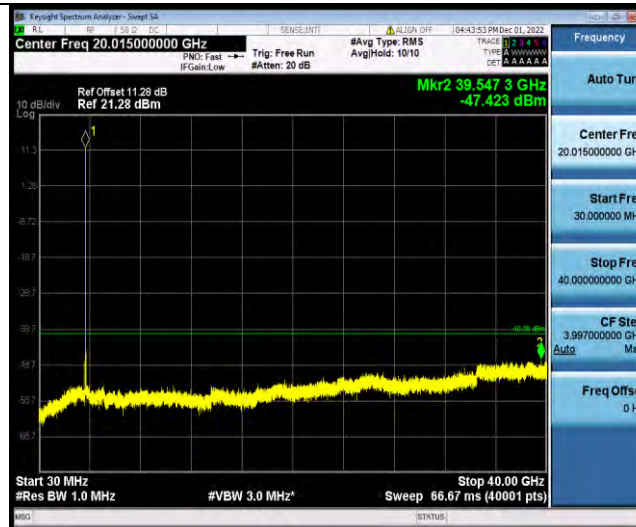
Band48-10MHz-16QAM-55290-1RB#0-Range1:30~40000MHz
