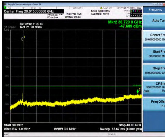
Band48-15MHz-QPSK-55315-1RB#0-Range1:30~40000MHz
