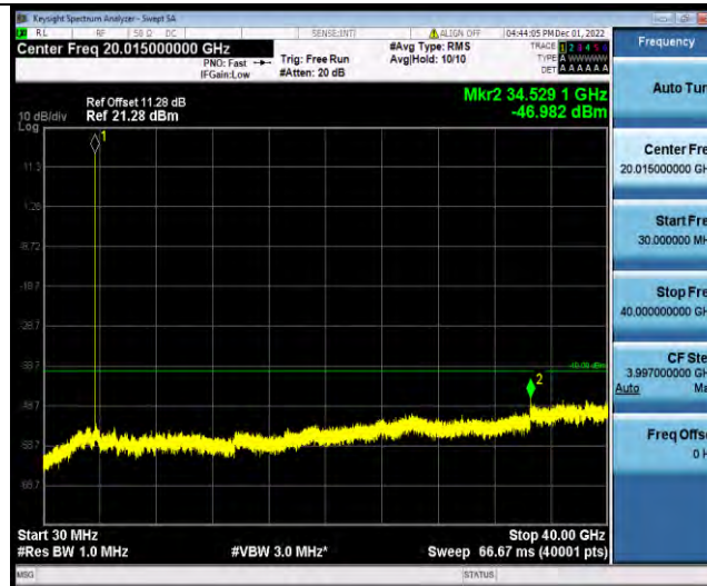
Band48-10MHz-64QAM-55290-1RB#0-Range1:30~40000MHz
