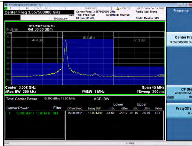
Band48-15MHz-QPSK-55315-75RB#0
