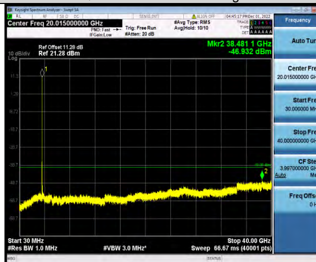
Band48-15MHz-QPSK-56665-1RB#0-Range1:30~40000MHz
