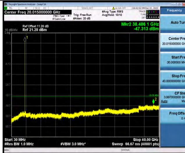
Band48-5MHz-64QAM-55265-1RB#0-Range1:30~40000MHz
