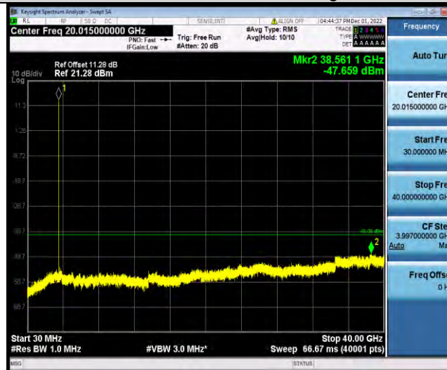
Band48-15MHz-QPSK-55990-1RB#0-Range1:30~40000MHz
