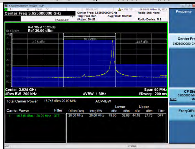
Band48-20MHz-QPSK-55990-100RB#0
