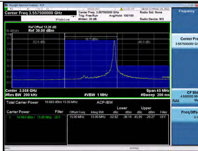
Band48-15MHz-QPSK-55990-1RB#0
