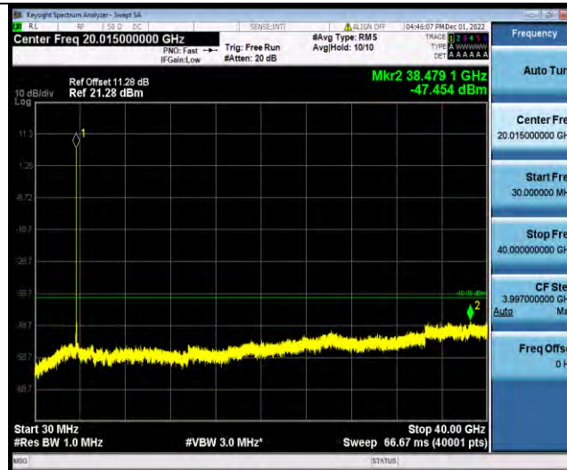
Band48-15MHz-64QAM-55315-1RB#0-Range1:30~40000MHz
