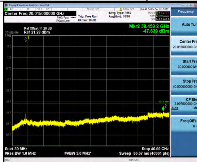
Band48-10MHz-QPSK-55990-1RB#0-Range1:30~40000MHz
