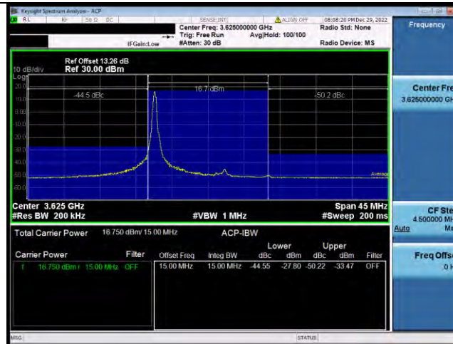
Band48-15MHz-QPSK-55990-75RB#0
