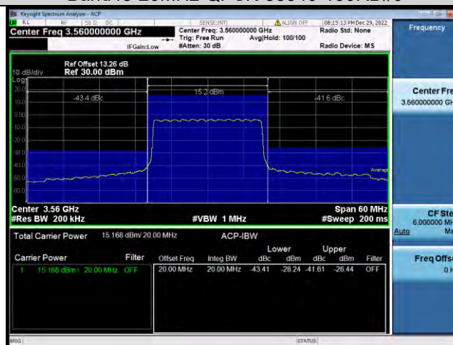
Band48-20MHz-QPSK-55990-1RB#0
