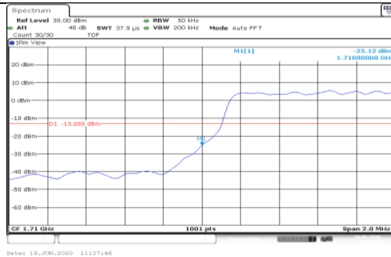
Band66-3MHz-QPSK-132657-1RB#14
