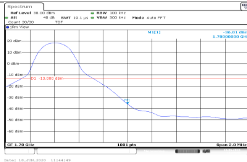
Band66-10MHz-16QAM-132622-50RB#0
