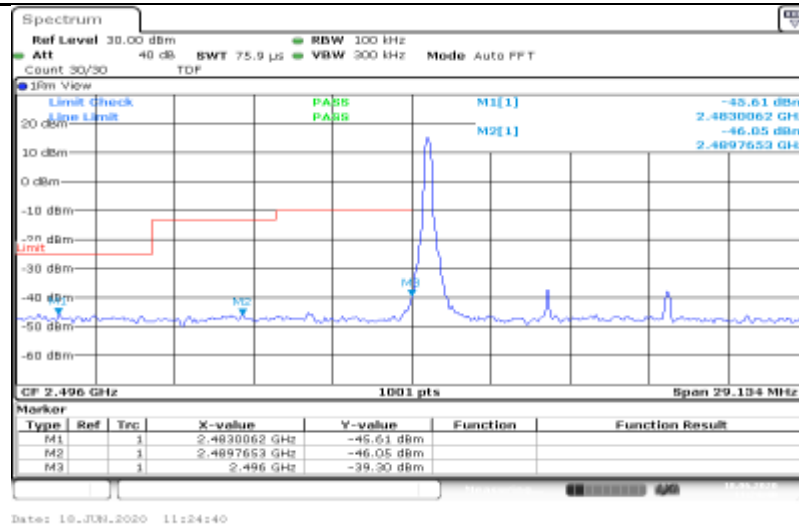
Band41-10MHz-16QAM-39700-50RB#0
