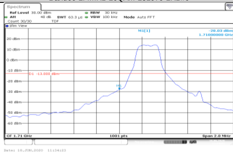
Band66-1.4MHz-16QAM-131979-6RB#0
