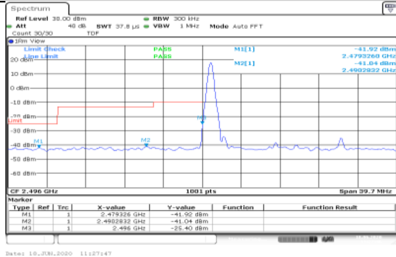
Band41-15MHz-QPSK-39725-75RB#0
