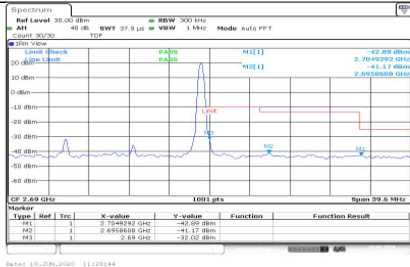
Band41-15MHz-QPSK-41515-75RB#0
