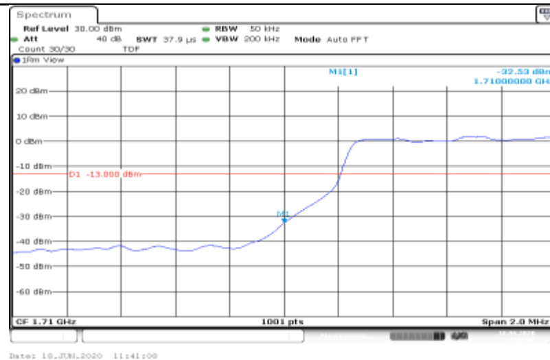
Band66-5MHz-16QAM-132647-1RB#24
