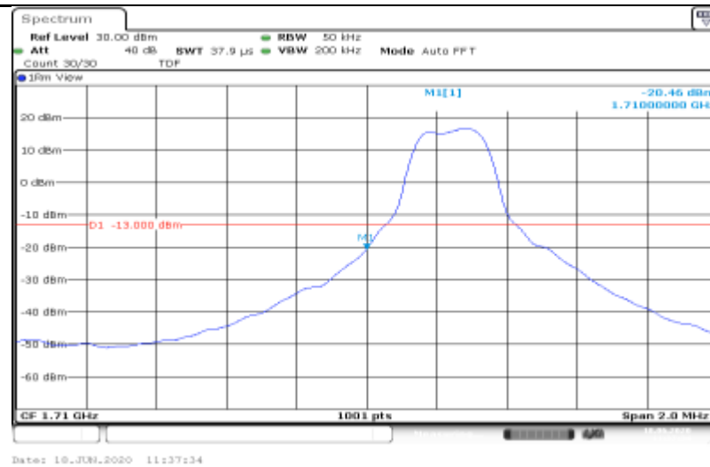
Band66-3MHz-16QAM-131987-15RB#0
