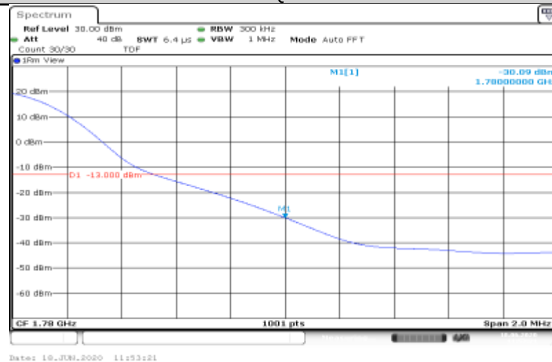
Band66-20MHz-16QAM-132572-100RB#0
