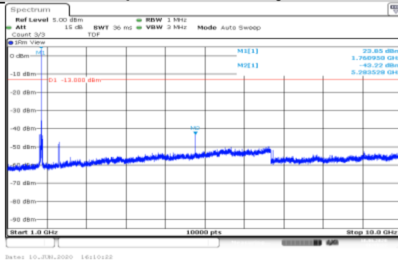
Band66-20MHz-16QAM-132572-1RB#0-Range2:1000~10000MHz
