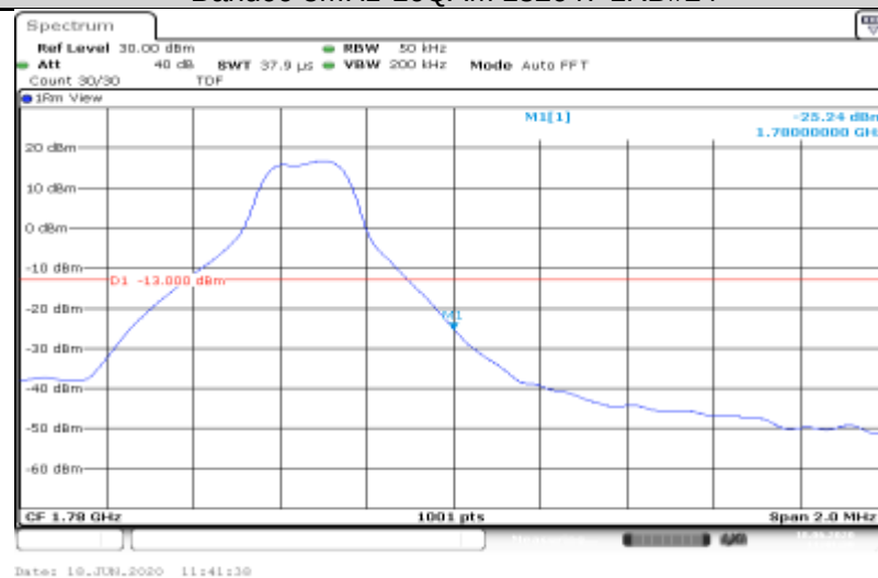
Band66-5MHz-16QAM-132647-25RB#0
