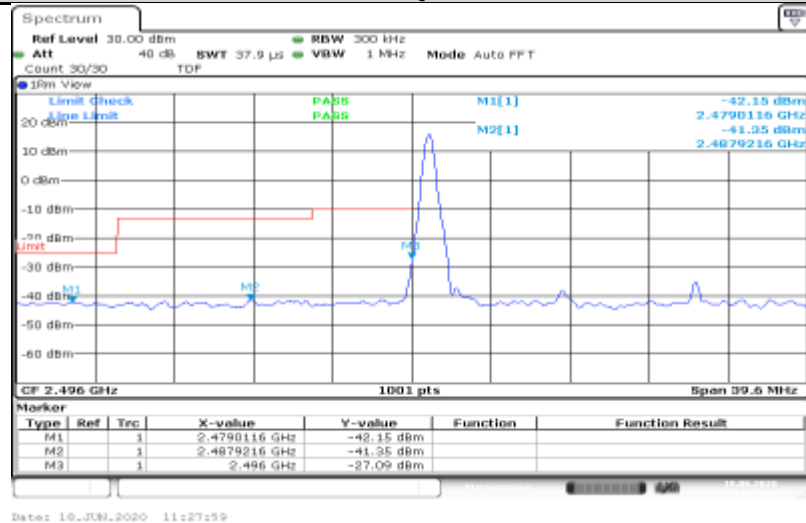
Band41-15MHz-16QAM-39725-75RB#0
