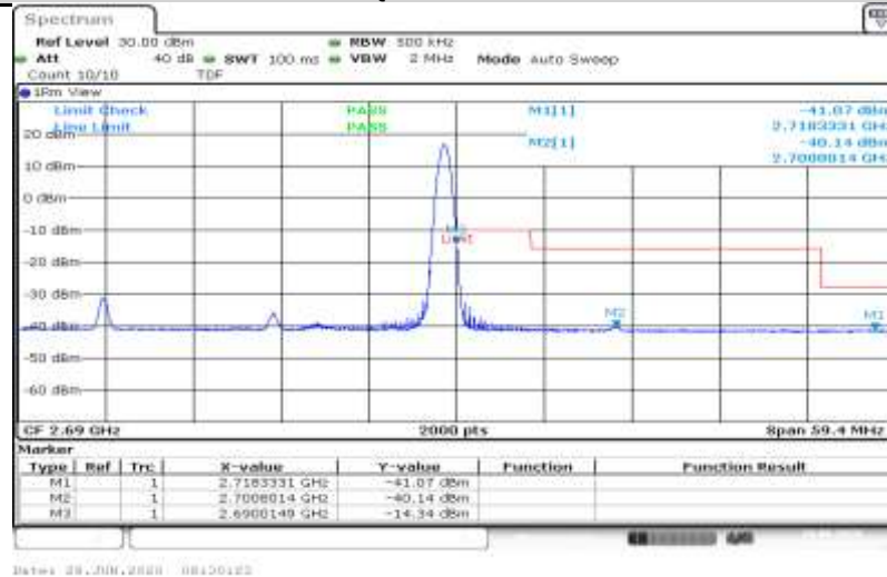
41-41-10MHz-15MHz-QPSK-41395-41515-50RB#0-75RB#0
