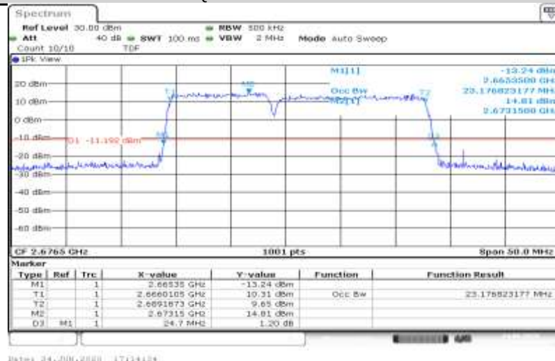
41-41-10MHz-15MHz-16QAM-39703-39823-50RB#0-75RB#0-23.177
