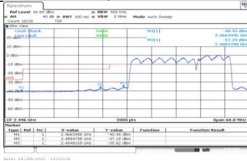
41-41-20MHz-10MHz-16QAM-39750-39894-1RB#0-0RB#0
