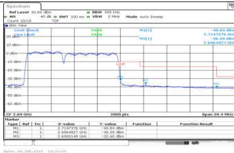
41-41-10MHz-15MHz-16QAM-39703-39823-1RB#0-0RB#0
