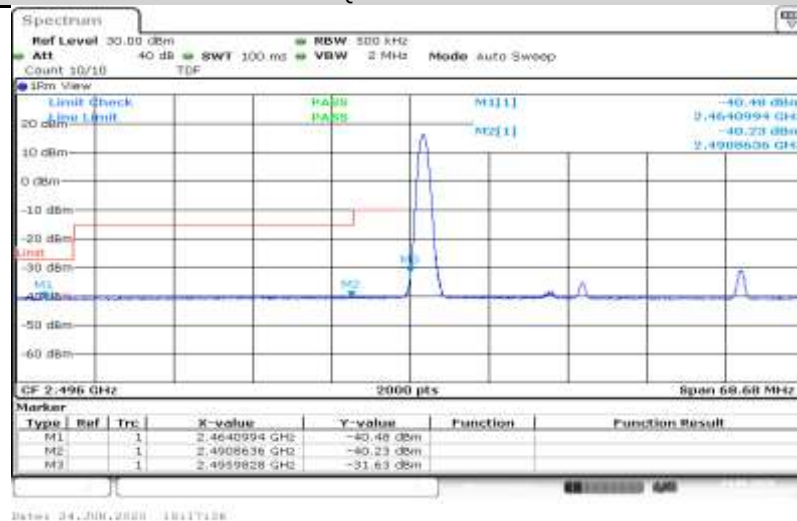
41-41-20MHz-10MHz-QPSK-41391-41535-0RB#0-1RB#49
