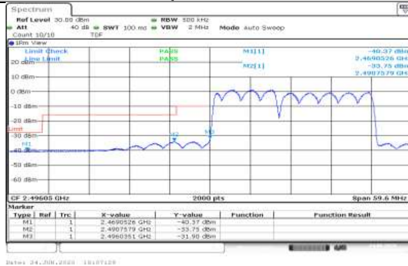
41-41-10MHz-15MHz-QPSK-41395-41515-0RB#0-1RB#74
