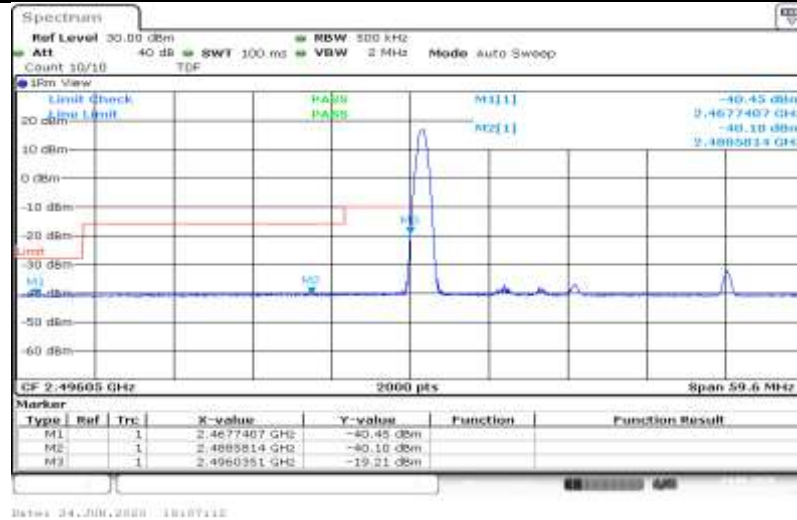
41-41-10MHz-15MHz-QPSK-39703-39823-50RB#0-75RB#0
