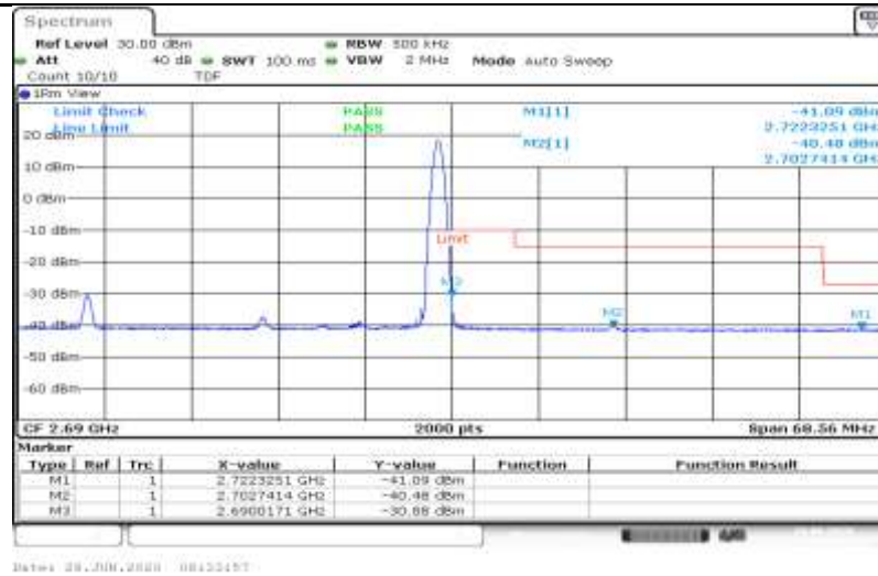
41-41-20MHz-10MHz-QPSK-41391-41535-100RB#0-50RB#0
