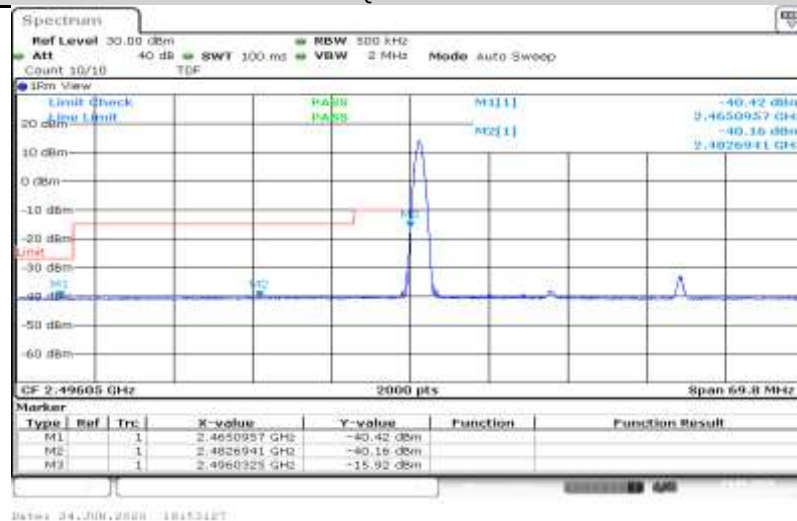
41-41-10MHz-15MHz-16QAM-39703-39823-50RB#0-75RB#0
