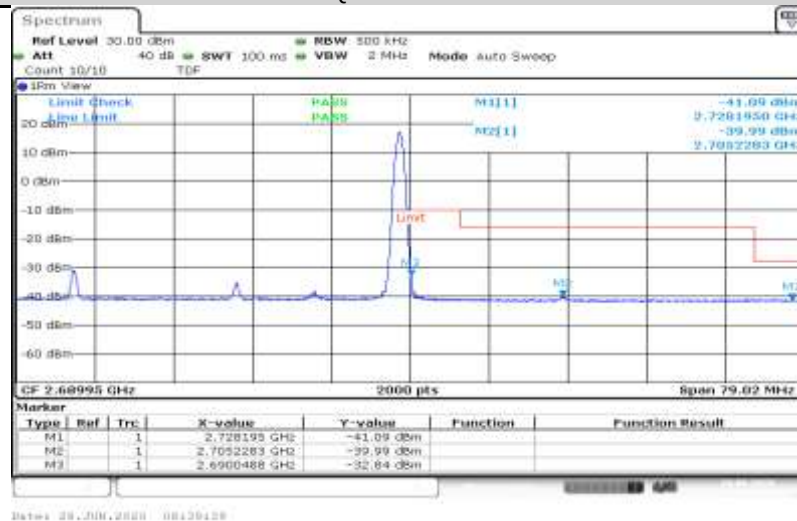
41-41-20MHz-15MHz-QPSK-41341-41512-100RB#0-75RB#0
