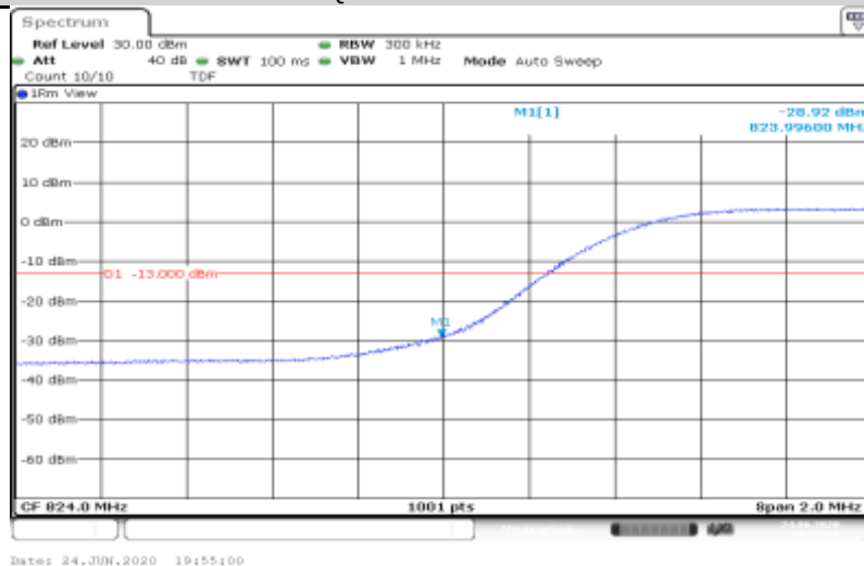
5-5-10MHz-5MHz-QPSK-20550-20622-0RB#0-1RB#24
