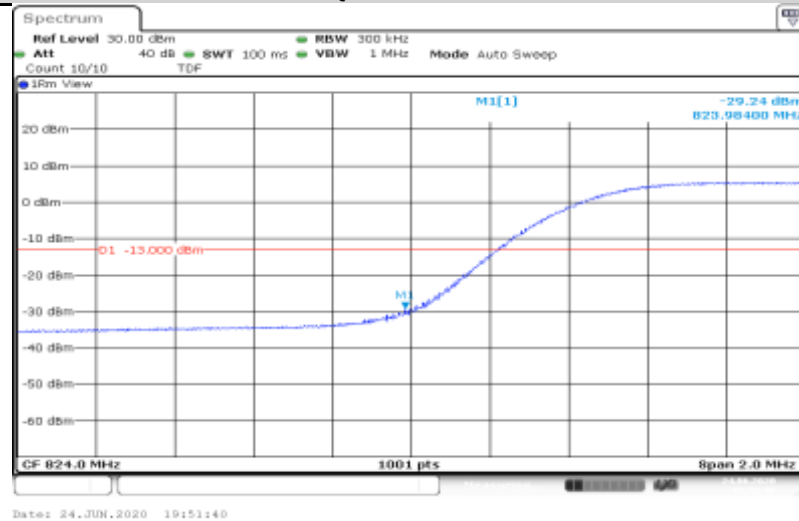
5-10MHz-10MHz-16QA M-20501-20600-0RB#0-1RB#49
