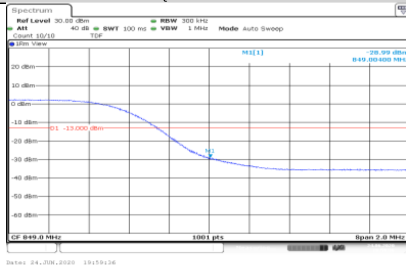
5-5-10MHz-10MHz-16QAM-20450-20549-1RB#0-0RB#0
