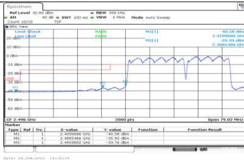
41-41-20MHz-15MHz-QPSK-39750-39921-1RB#0-0RB#0
