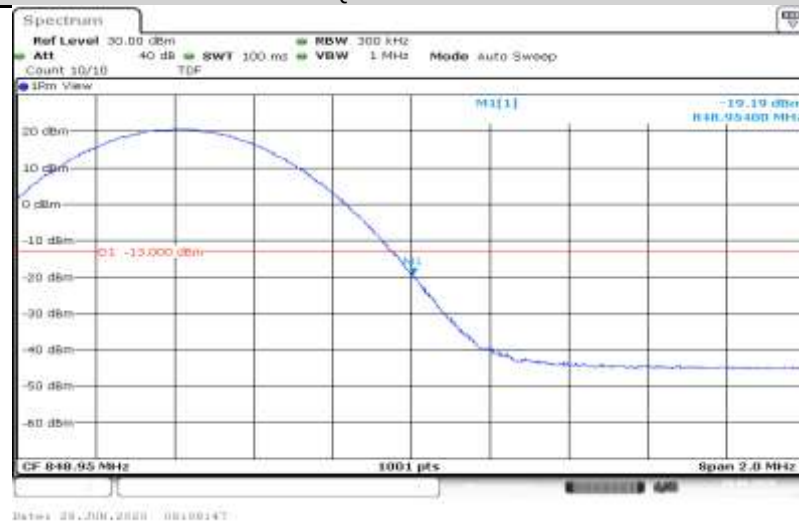
5-5-10MHz-5MHz-16QA M-20550-20622-50RB#0-25RB#0
