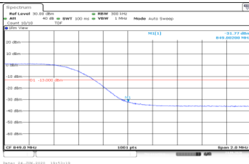
5-5-10MHz-5MHz-QPSK-20450-20522-1RB#0-0RB#0
