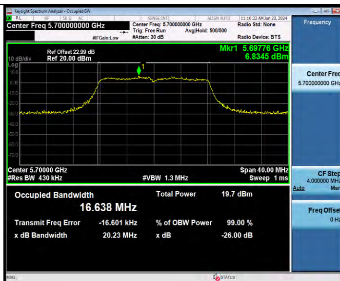
11A-CDD Ant2 5700
