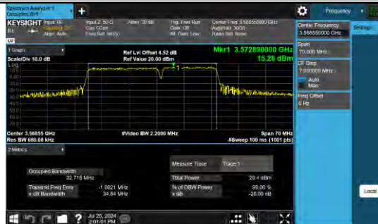
48-48-20MHz-15MHz-QPSK-QPSK-55340-55511-100RB #0-75RB#0-PASS
