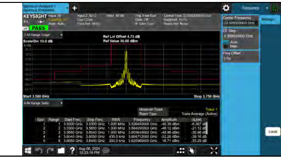
48-48-20MHz-20MHz-QPSK@QPSK-QPSK@QPSK-558 91-56089-1RB#99@100RB#0-1RB#0@100RB#0-PASS
