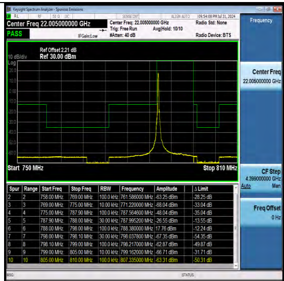
NTNV-N14-PC2-15-10-M-DFT-QPSK-Edge_1RB_Left-Ant1-PASS
