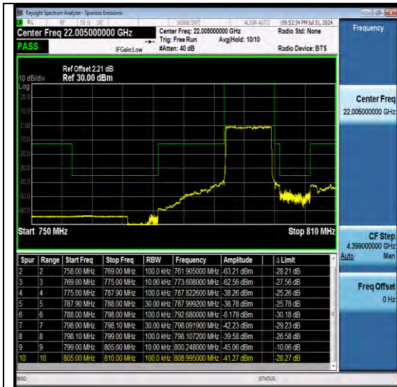
NTNV-N14-PC2-15-10-M-DFT-QPSK-Outter_Full-Ant1-PASS
