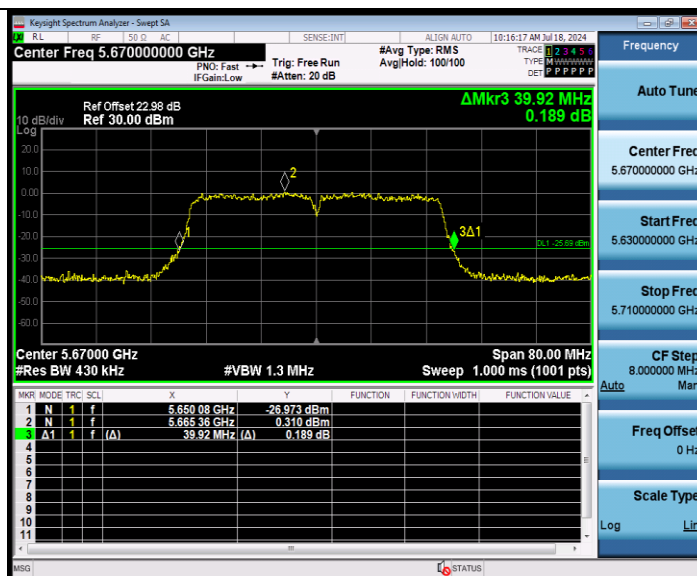
11N40MIMO Ant2 5670
