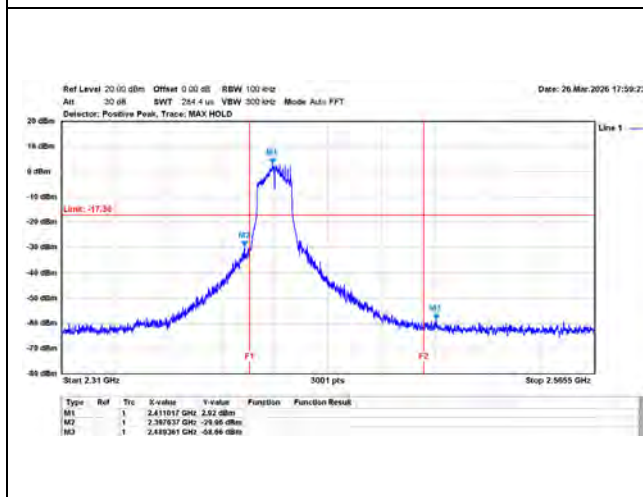
802.11n/20MHz/MCS0/2412MHz/Ch1/Ant.1(Band Edge)
