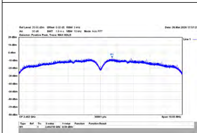
802.11b/20MHz/1M/2462MHz/Ch11/Ant.1
