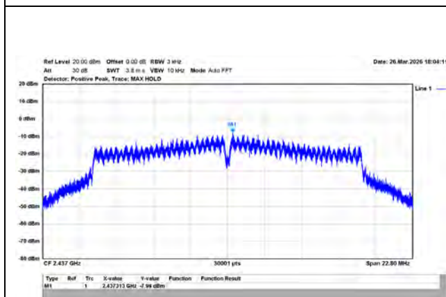
802.11g/20MHz/6M/2437MHz/Ch6/Ant.1
