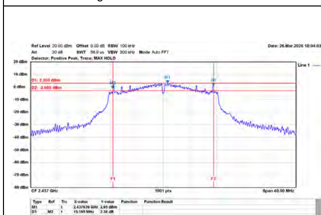
802.11g/20MHz/6M/2437MHz/Ch6/Ant.1
