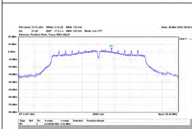
802.11n/20MHz/MCS0/2437MHz/Ch6/Ant.1 (Ref.)
