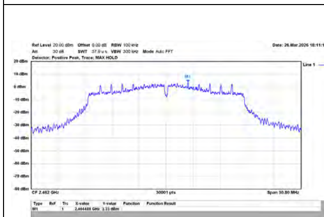
802.11n/20MHz/MCS0/2462MHz/Ch11/Ant.1 (Ref.)
