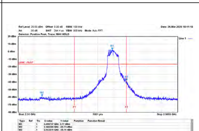
802.11n/20MHz/MCS0/2462MHz/Ch11/Ant.1(Band Edge)
