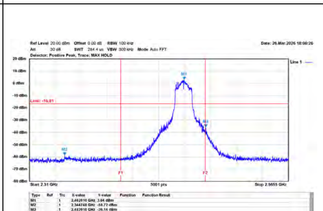
802.11g/20MHz/6M/2462MHz/Ch11/Ant.1(Band Edge)
