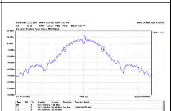
802.11b/20MHz/1M/2437MHz/Ch6/Ant.1
