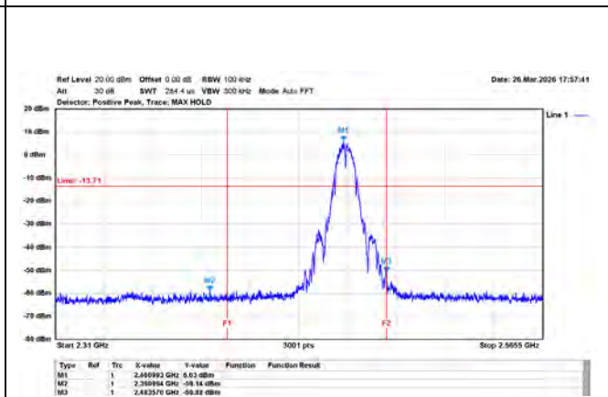
802.11b/20MHz/1M/2462MHz/Ch11/Ant.1(Band Edge)
