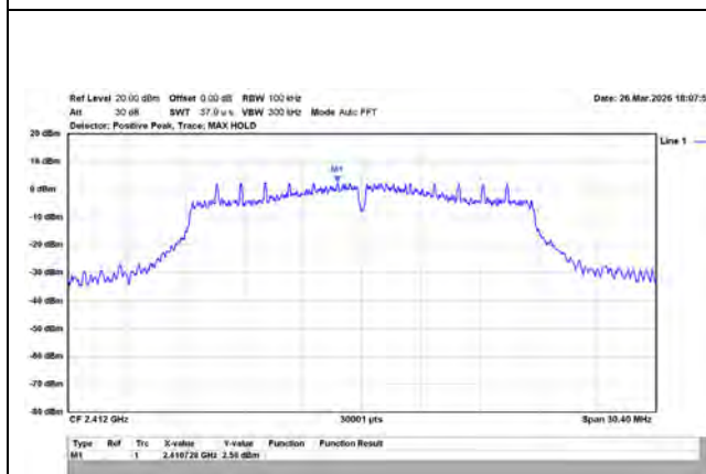
802.11n/20MHz/MCS0/2412MHz/Ch1/Ant.1 (Ref.)
