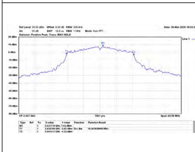
802.11g/20MHz/6M/2437MHz/Ch6/Ant.1
