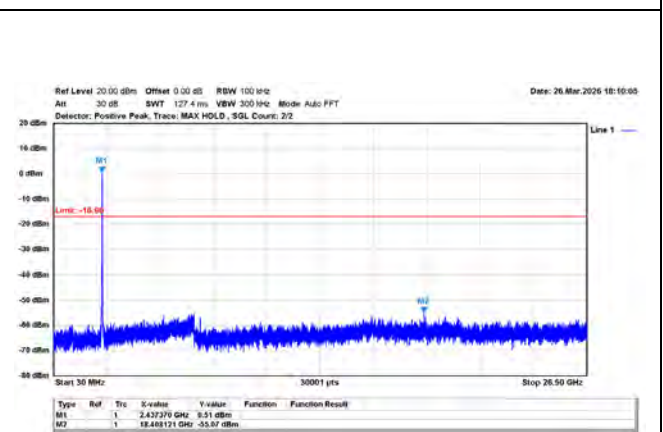
802.11n/20MHz/MCS0/2437MHz/Ch6/Ant.1
