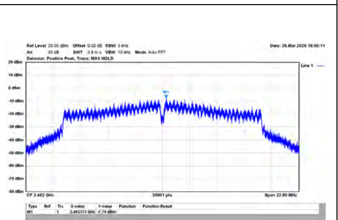
802.11g/20MHz/6M/2462MHz/Ch11/Ant.1
