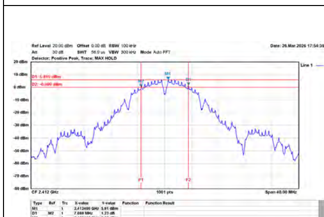
802.11b/20MHz/1M/2412MHz/Ch1/Ant.1
