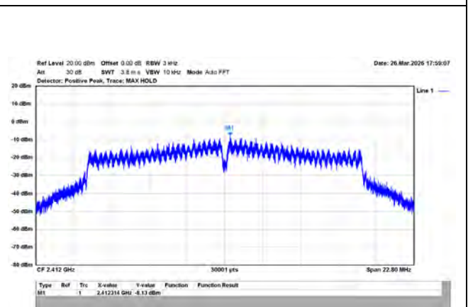
802.11g/20MHz/6M/2412MHz/Ch1/Ant.1
