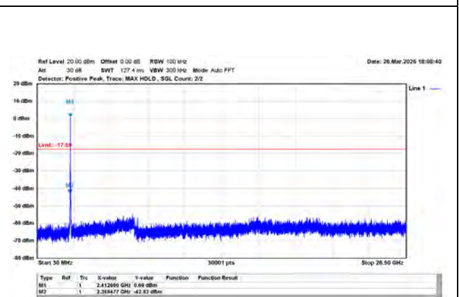
802.11n/20MHz/MCS0/2412MHz/Ch1/Ant.1
