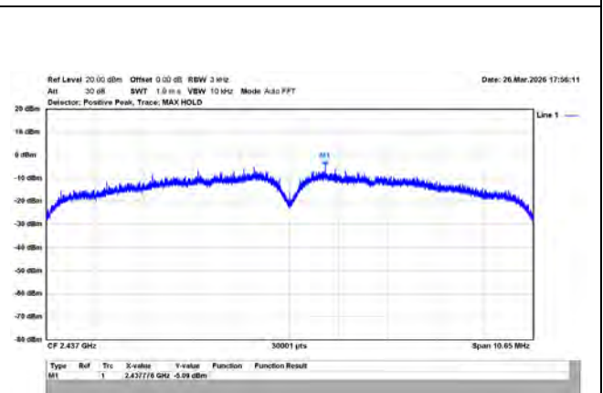
802.11b/20MHz/1M/2437MHz/Ch6/Ant.1
