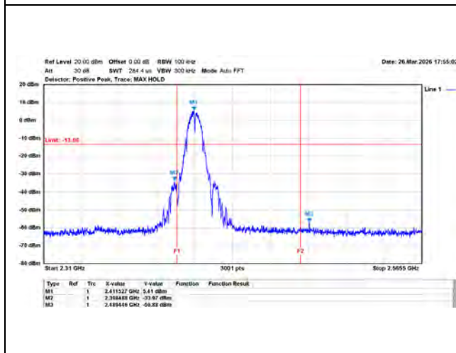
802.11g/20MHz/6M/2412MHz/Ch1/Ant.1(Band Edge)
