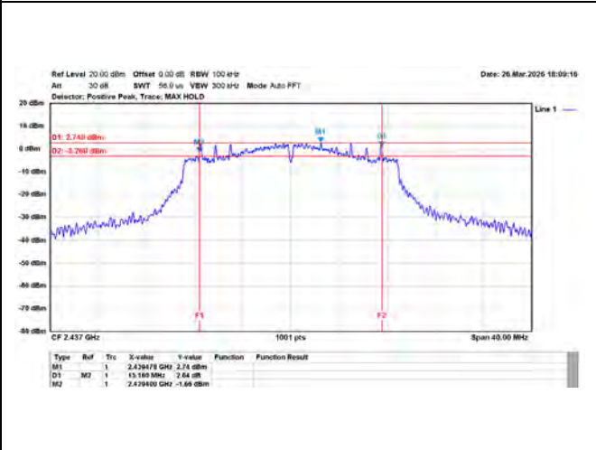
802.11n/20MHz/MCS0/2437MHz/Ch6/Ant.1
