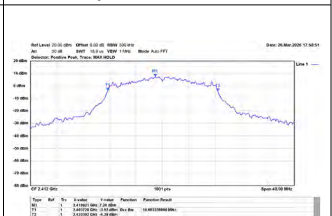
802.11g/20MHz/6M/2412MHz/Ch1/Ant.1
