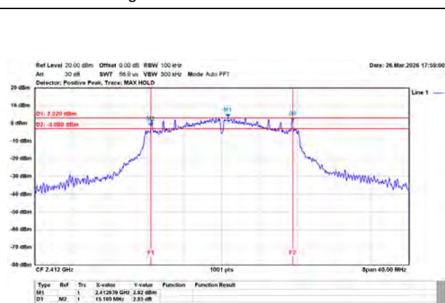
802.11g/20MHz/6M/2412MHz/Ch1/Ant.1
