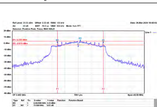
802.11g/20MHz/6M/2462MHz/Ch11/Ant.1
