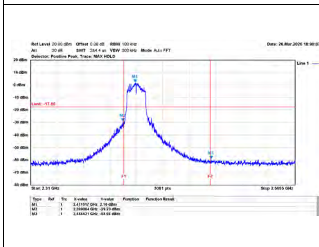
802.11n/20MHz/MCS0/2412MHz/Ch1/Ant.1(Band Edge)
