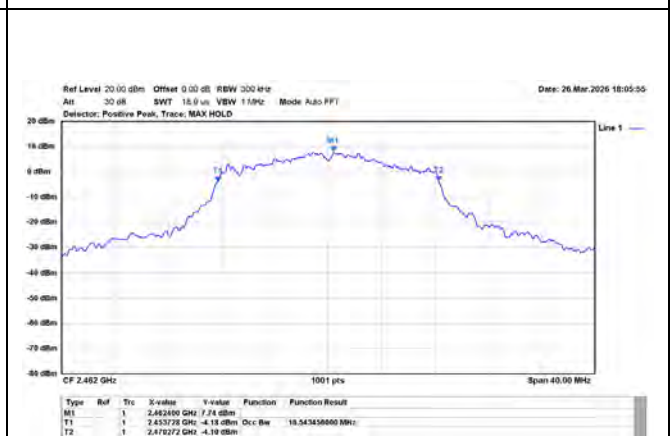
802.11g/20MHz/6M/2462MHz/Ch11/Ant.1
