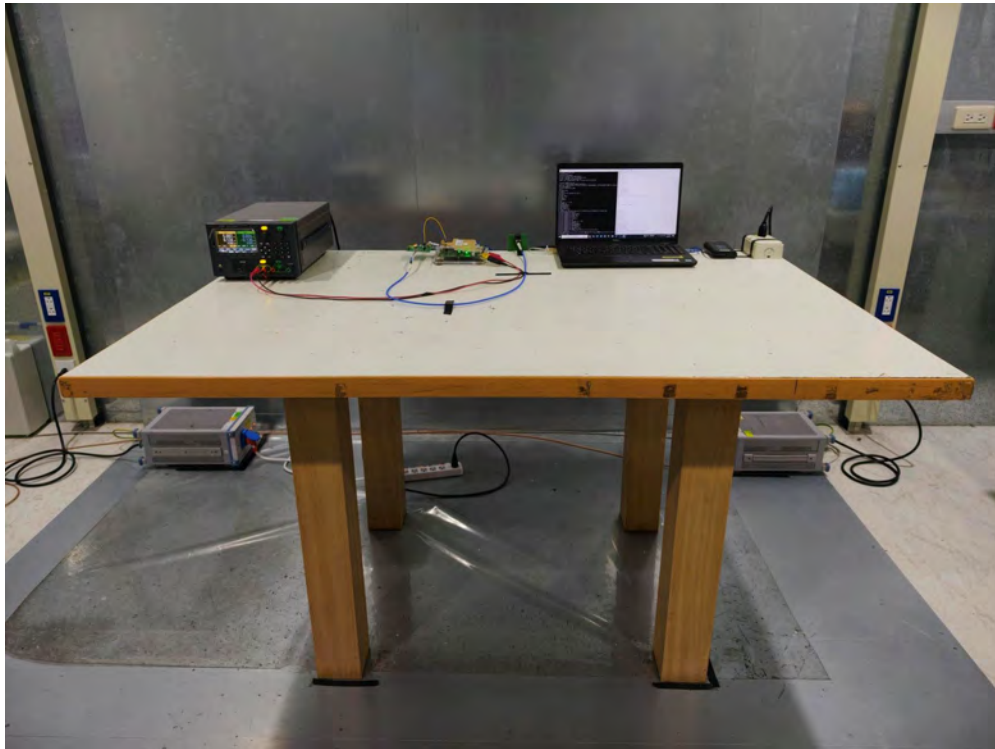
Front View of AC Power Line Conducted Emission Test
