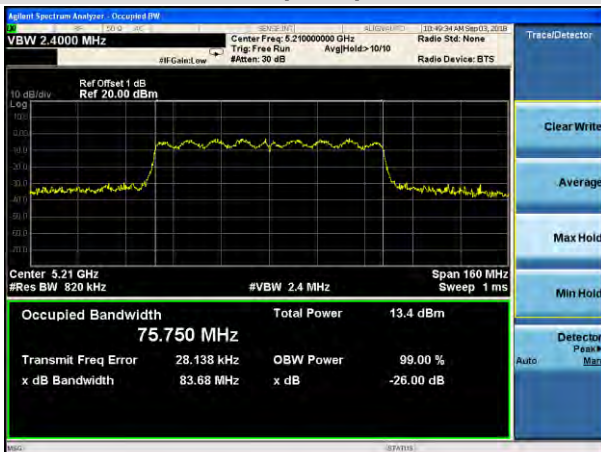
Channel 40 (5210MHz)
