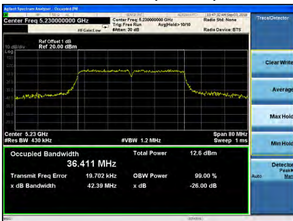
Channel 46 (5230MHz)
