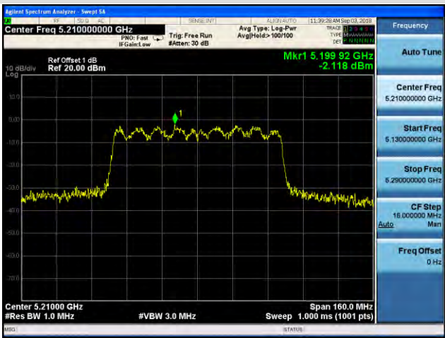
Channel 40 (5210MHz)
