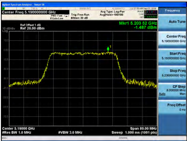
Channel 38 (5190MHz)
