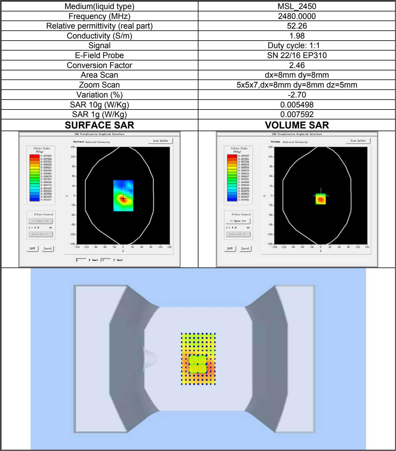
Plot 2:BT High channel (Body, Back side) Product Description: ROCAM mini HD-Basis Test Date: 2021-04-30
