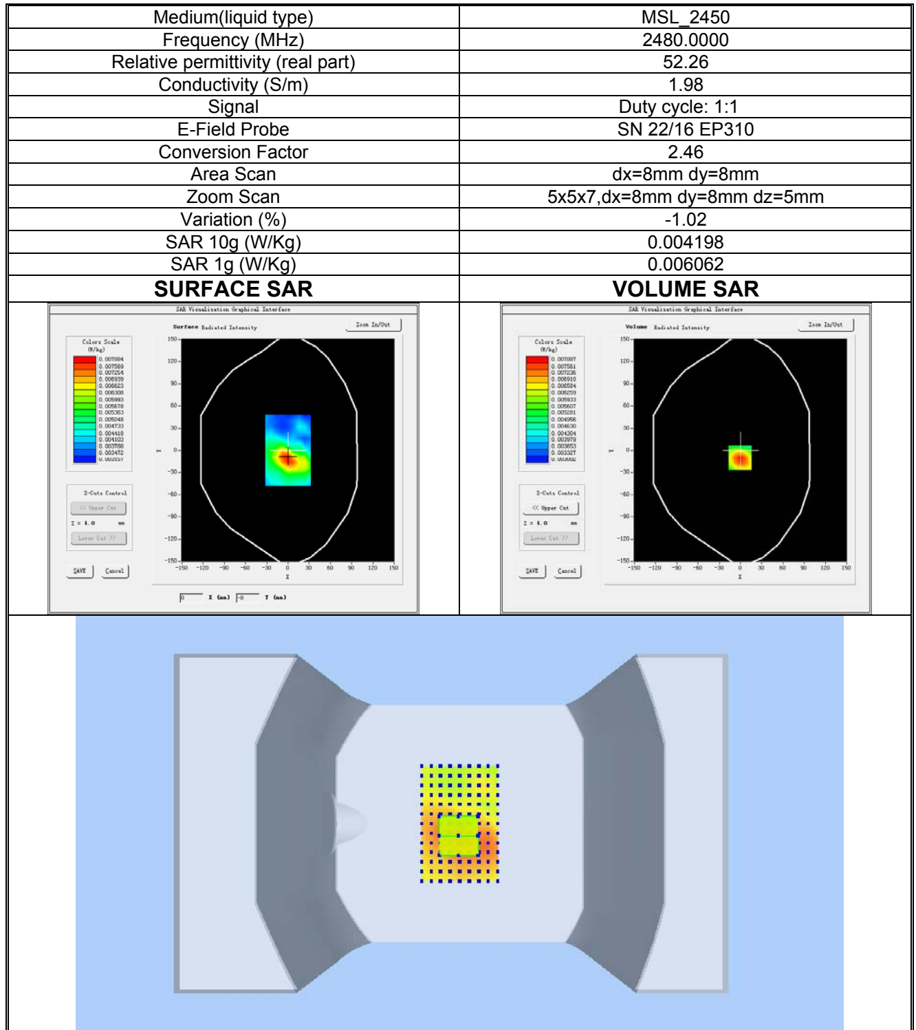
Plot 3: BLE High channel (Body, Back side) Product Description: ROCAM mini HD-Basis Test Date: 2021-04-30
