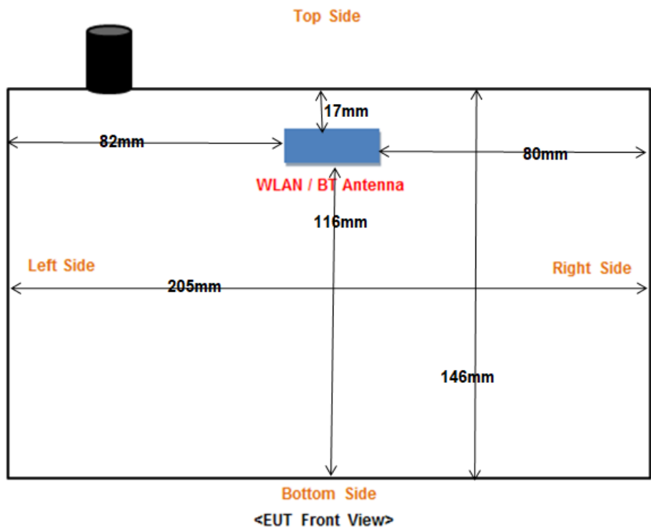
EUT Size: Long*Width*Height=205mm*146mm*67mm Fig 7.1 Block Diagram for EUT Antenna Position
