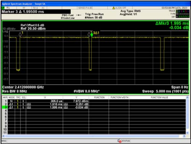
Wi-Fi 802.11n-HT20
