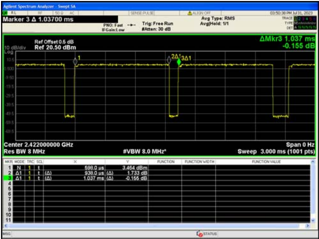
Wi-Fi 802.11n-HT40
