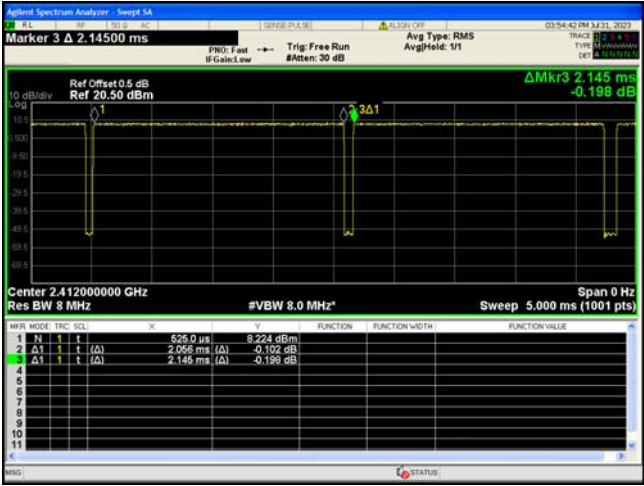
Wi-Fi 802.11g
