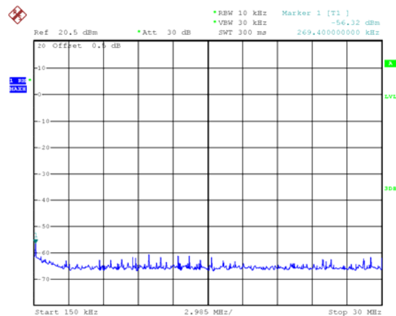
Mode: TX 11n20 channel 6
