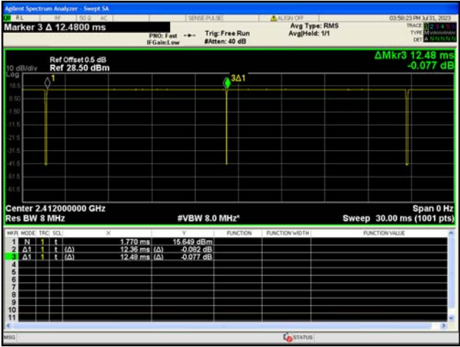
Wi-Fi 802.11b
